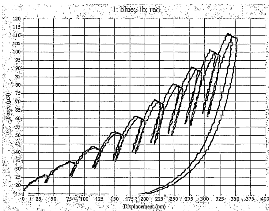
Figure 2. Typical force displacement curves for 2 comparative experiments of non – surface structured (flat) coating of formulation F showing good experimental reproducibility between the two curves.
