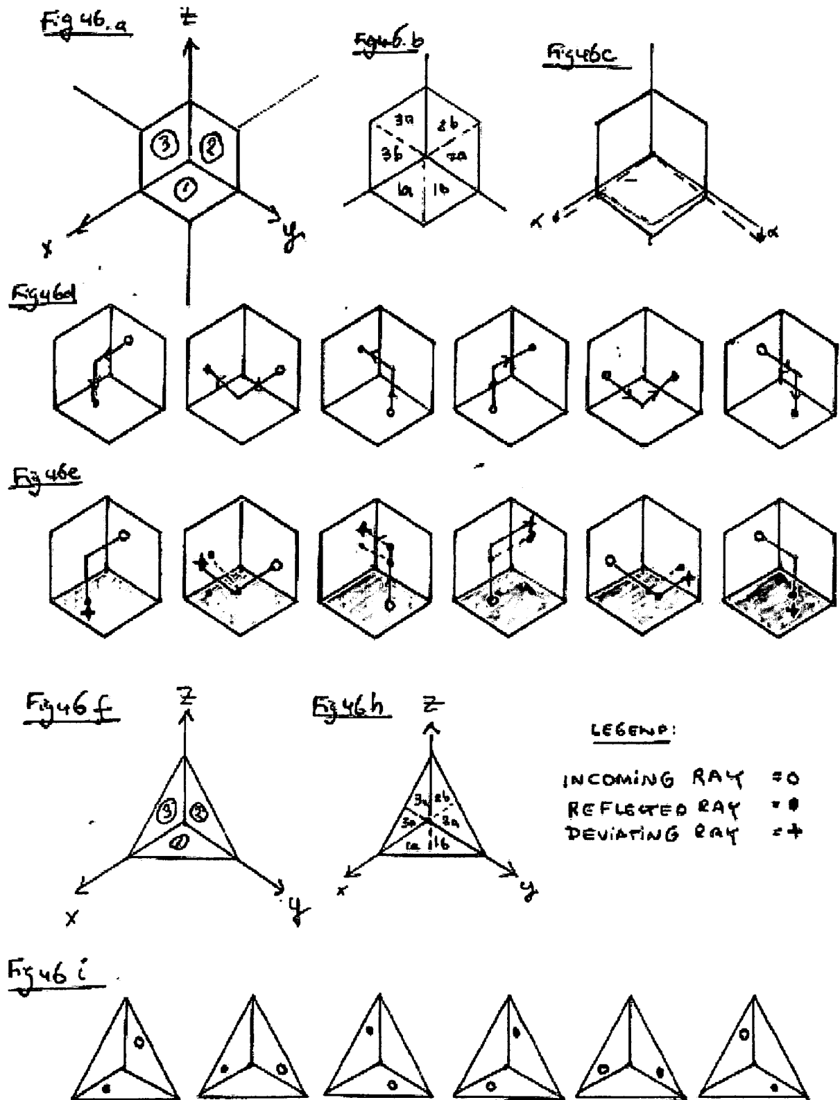
Figures 46a to 46i Retro reflecting structures with sub apertures (fig 46 c & e show alpha rotation of plane 1)
