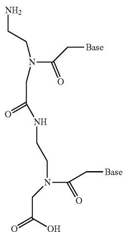
Peptide nucleic acid (PNA)
