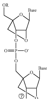
Locked nucleic acid
