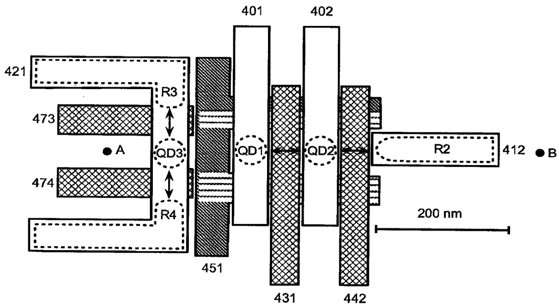
Figure 4B (PRIOR ART)
