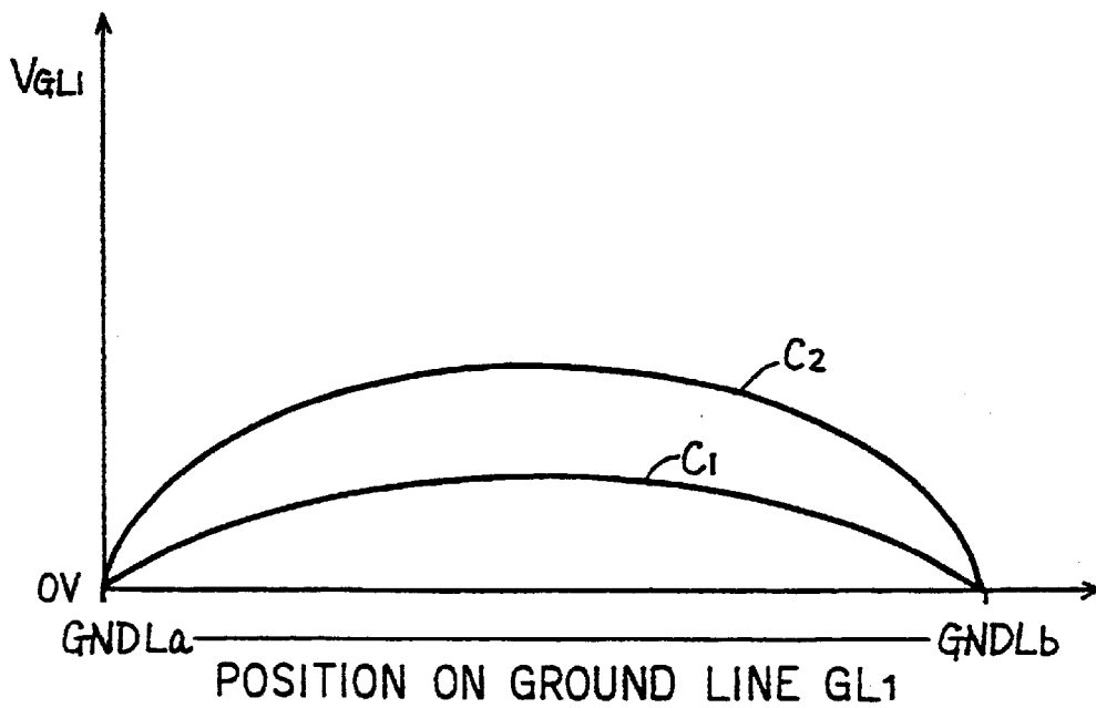
FIG. 19 PRIOR ART
