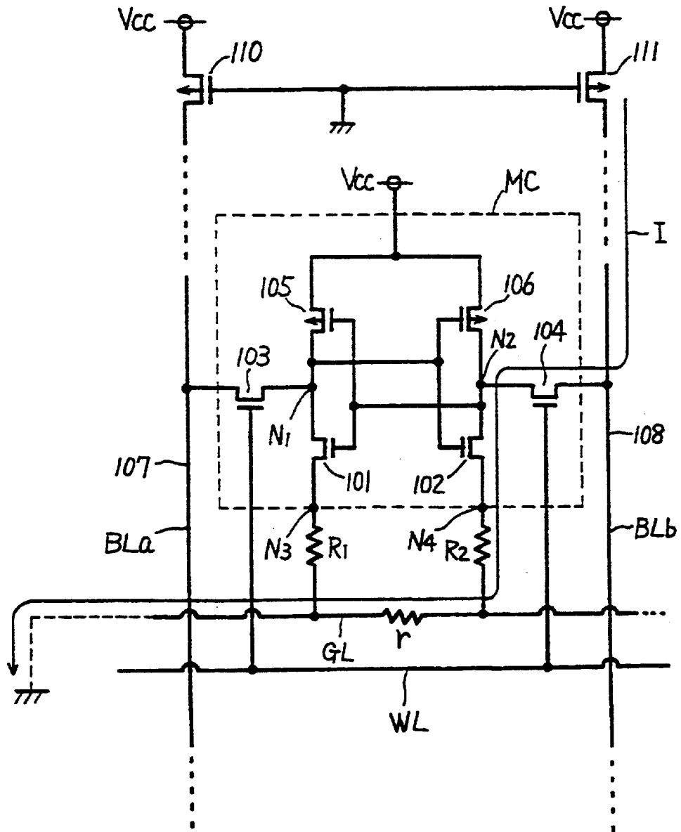
FIG. 14 PRIOR ART
