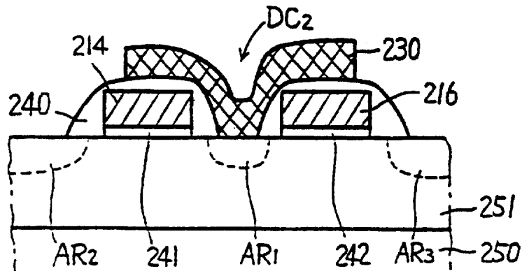
FIG. 17 PRIOR ART
