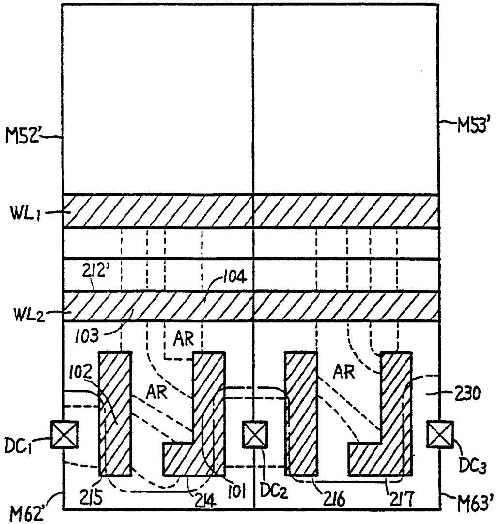
FIG. 16 PRIOR ART
