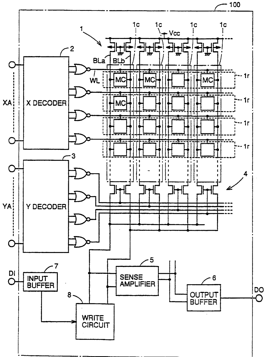
FIG. 13 PRIOR ART
