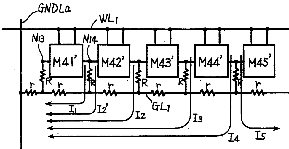
FIG. 18 PRIOR ART
