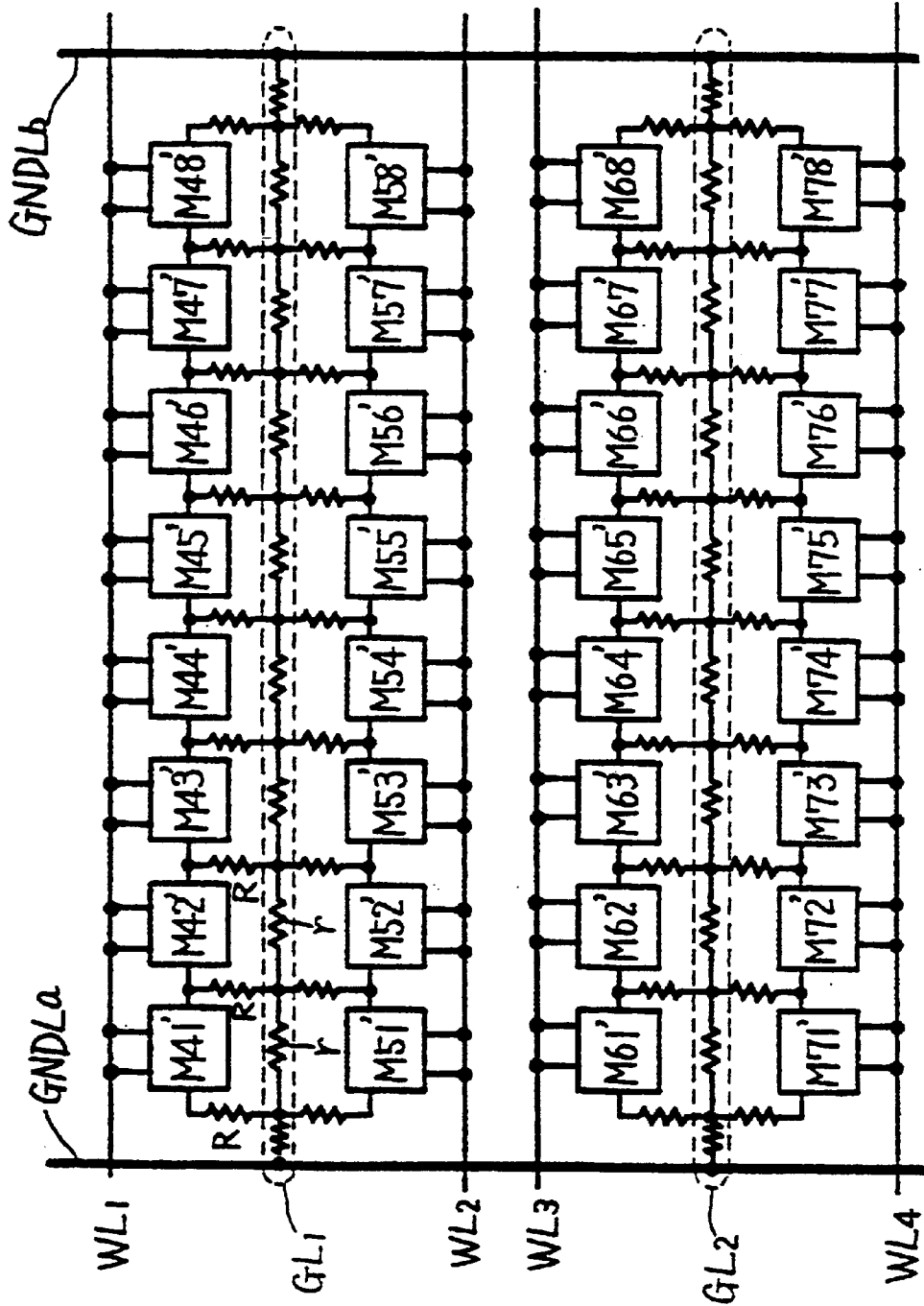
FIG. 15 PRIOR ART
