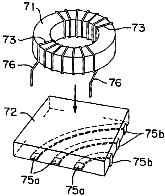
FIG. 12 PRIOR ART
