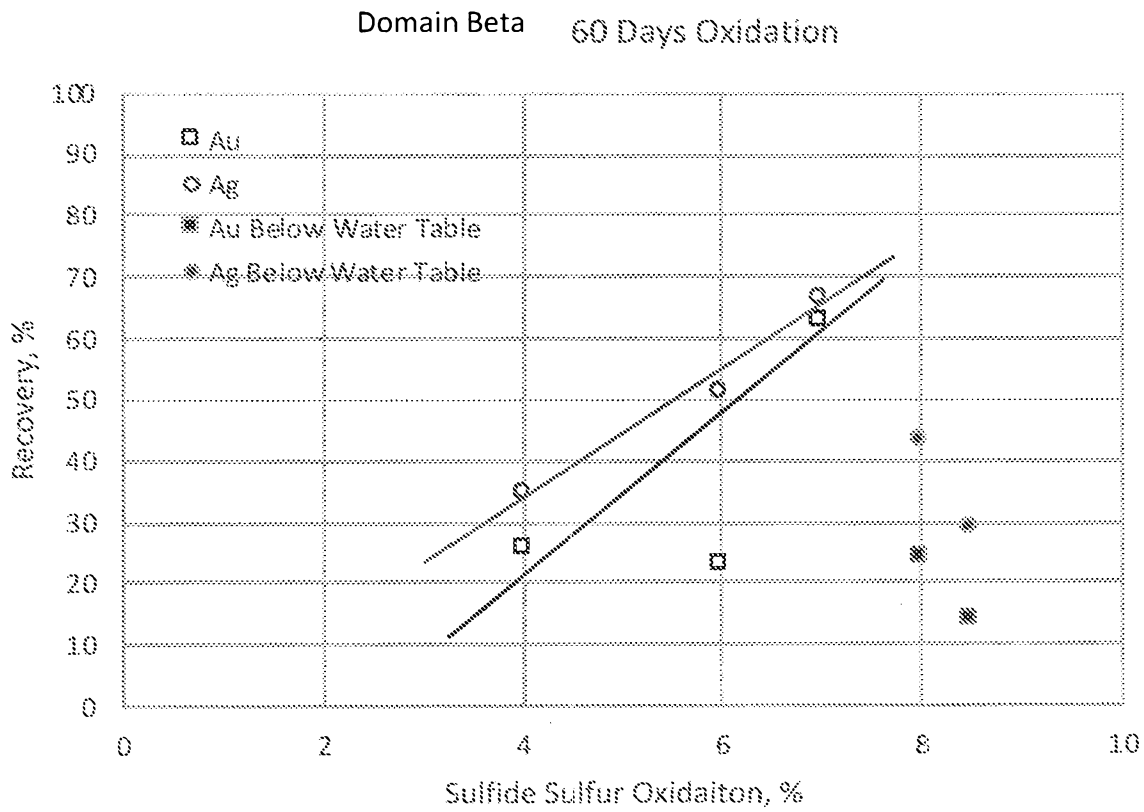
Effect of Oxidation on Leach Recovery Domain Beta Ore
