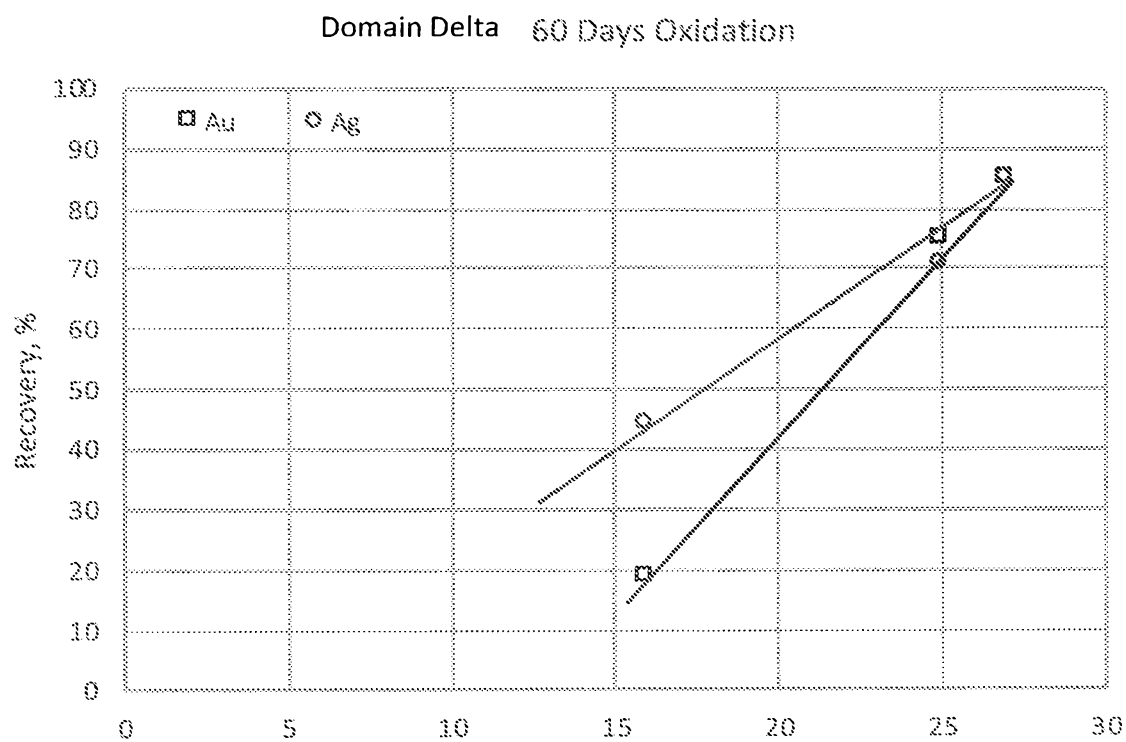
Effect of Oxidation on Leach Recovery – Domain Delta Ore
