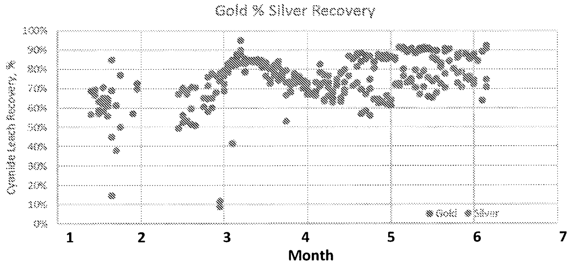
Figure 3 Demonstration Plant Cyanide Leach Recovery of Au and Ag
