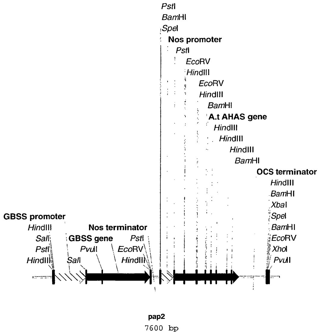
Fig 2. T-DNA of pAP2 construct
