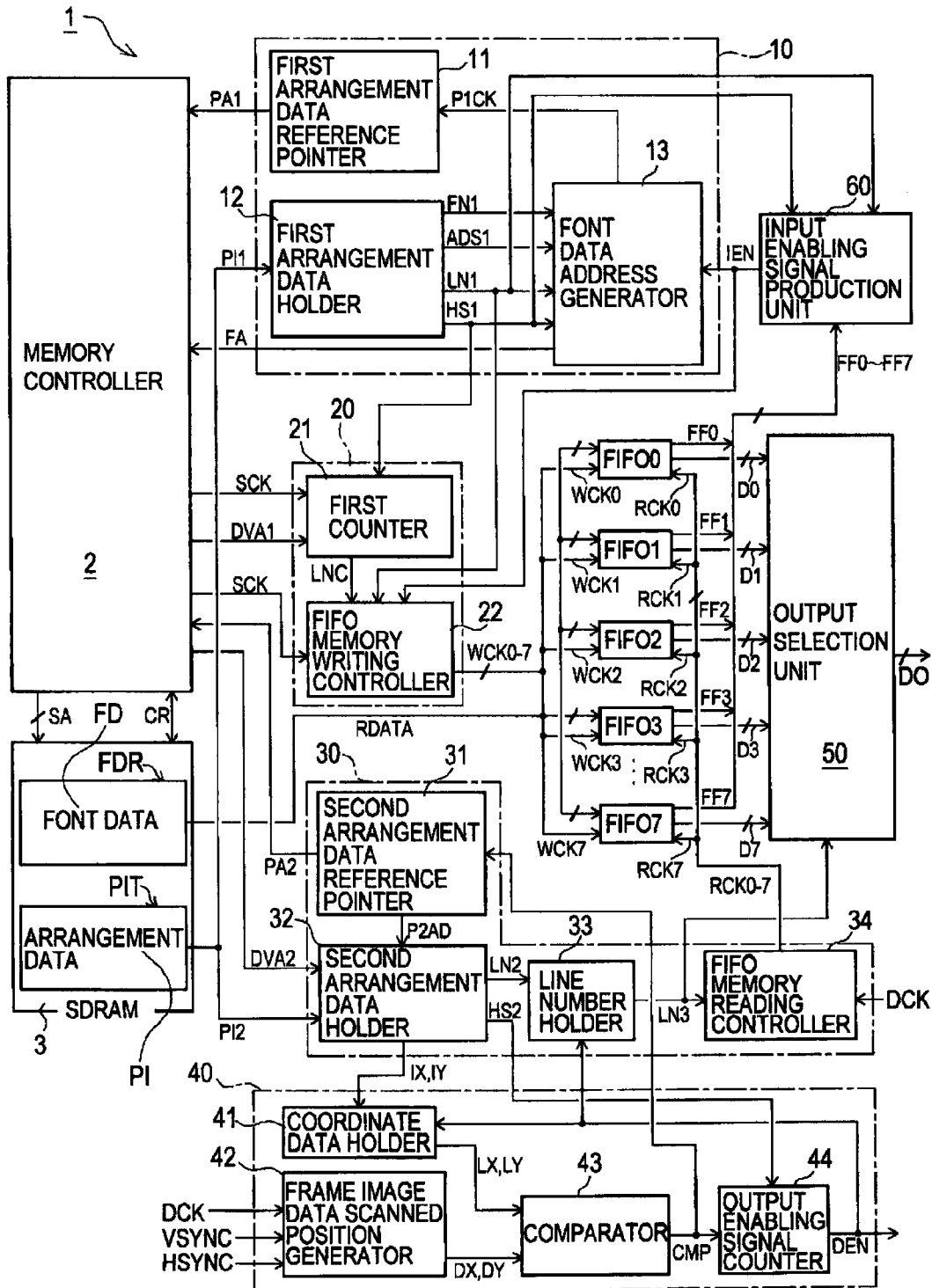
CIRCUITRY OF IMAGE DISPLAY SYSTEM IN ACCORDANCE WITH PRESENT EMBODIMENT
