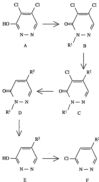
Scheme 1
