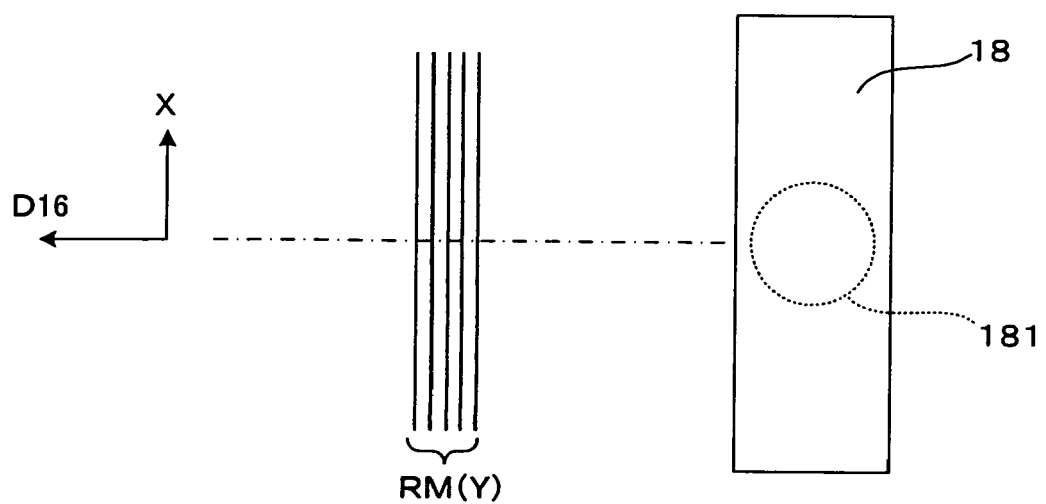
FIG. 11 B : ENLARGED PLAN VIEW OF REGISTRATION MARK
