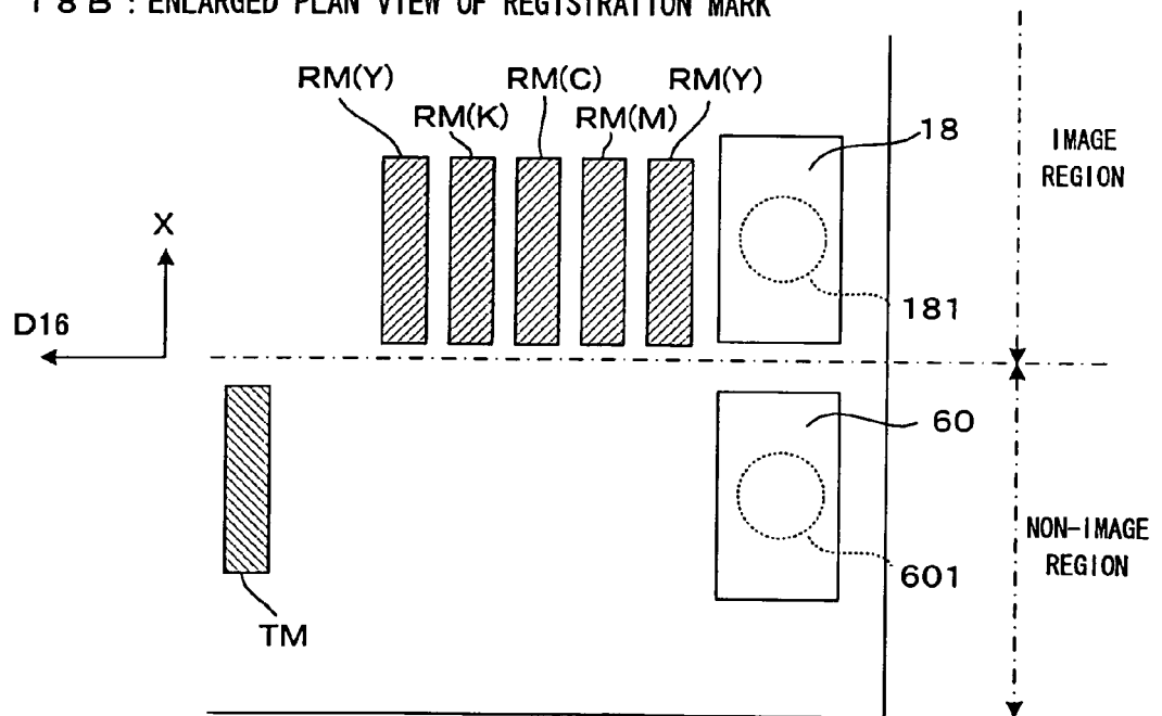
FIG. 18B : ENLARGED PLAN VIEW OF REGISTRATION MARK
