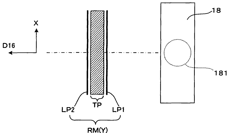
FIG. 5B : ENLARGED PLAN VIEW OF REGISTRATION MARK
