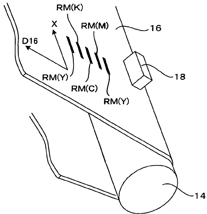
FIG. 5A : ENLARGED PERSPECTIVE VIEW OF SECTION NEAR SENSOR
