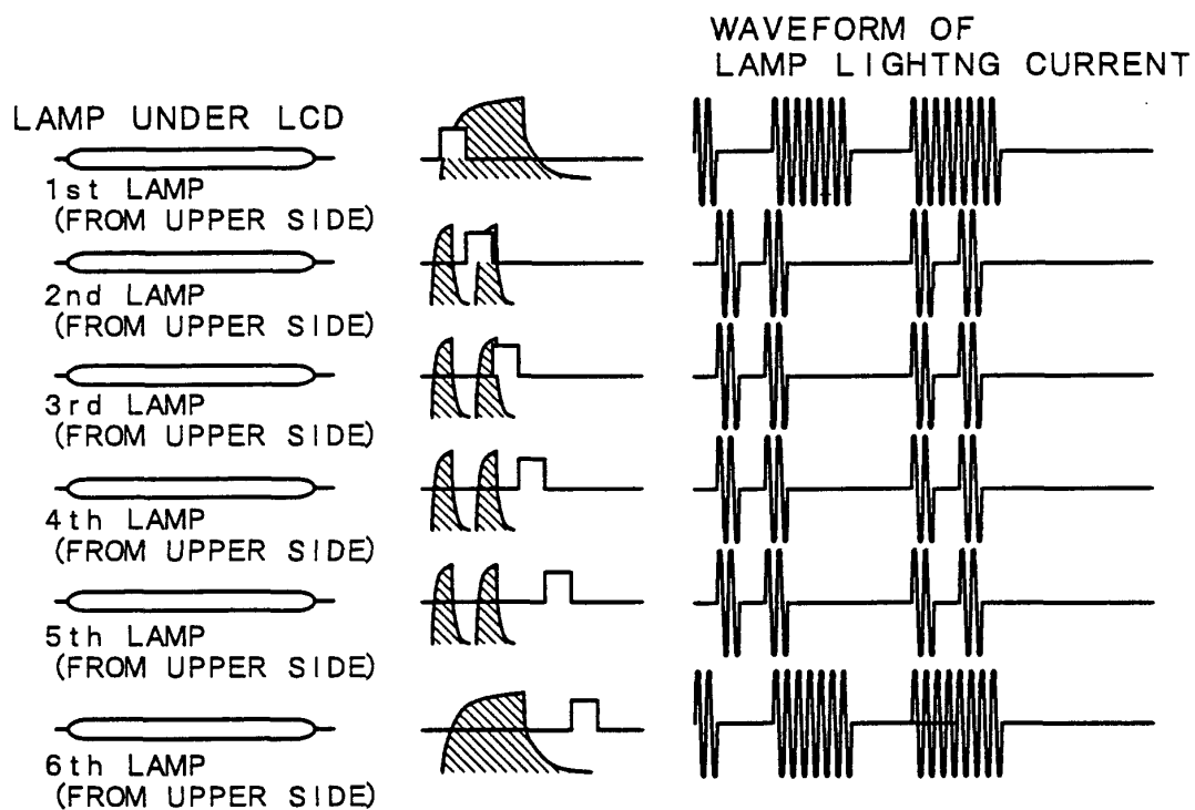
FIG. 27B LOW BRIGHTNESS WAVEFORM OF LAMP LIGHTING CURRENT
