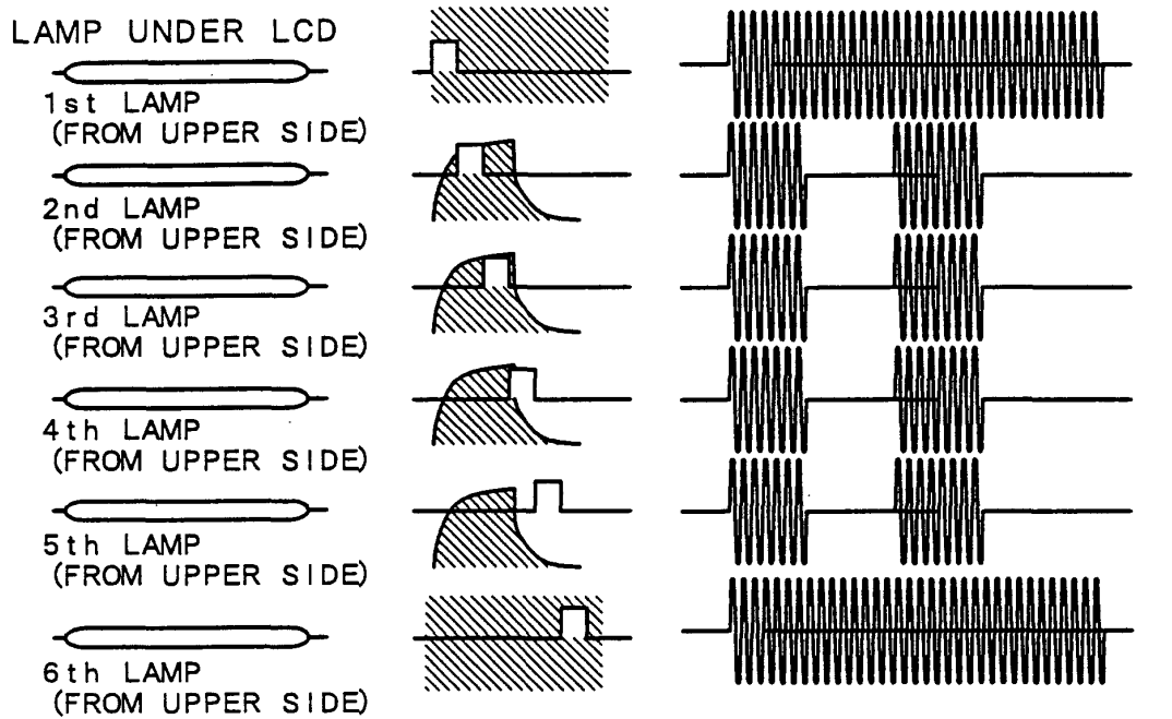
FIG. 27A HIGH BRIGHTNESS WAVEFORM OF LAMP LIGHTING CURRENT
