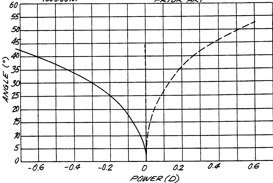
FIG. 59 PRIOR ART
