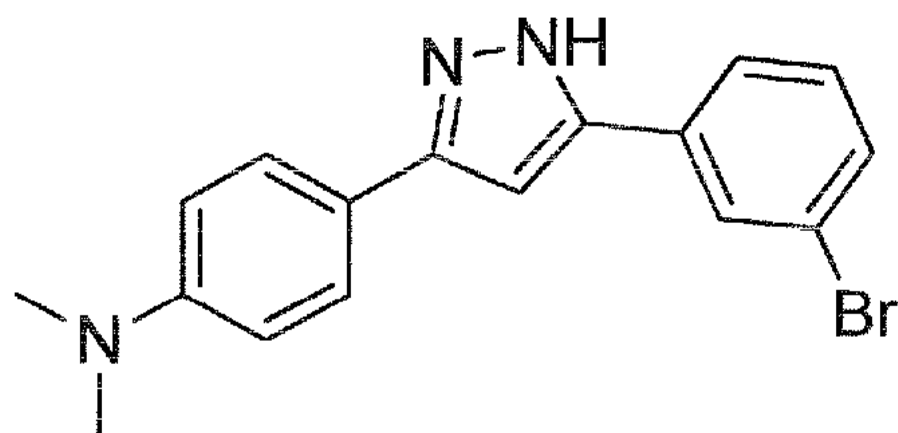
5-(3-Bromophenyl)-3-(4-dimethylaminophenyl)-1H-pyrazole
