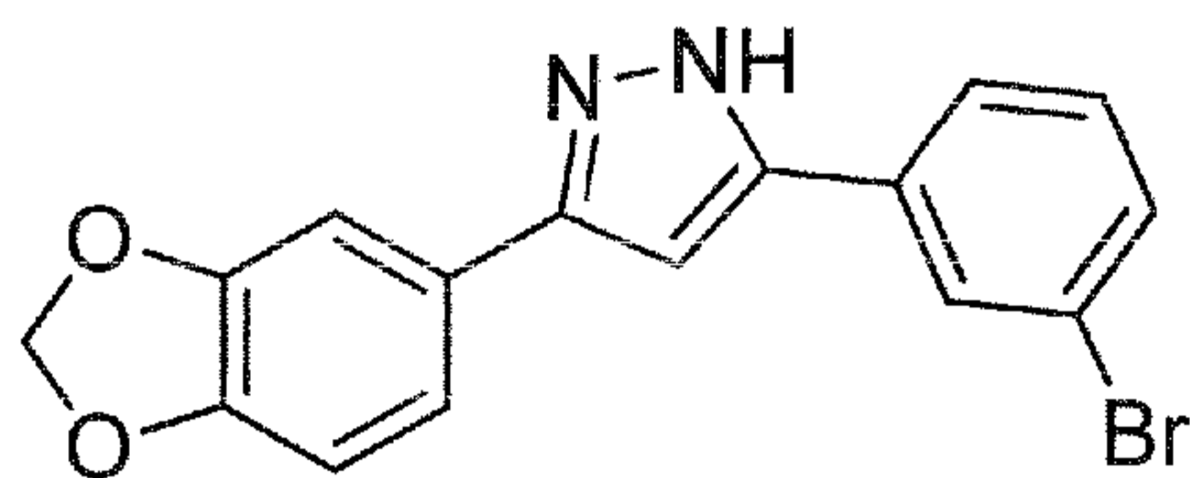
5-(3 -Bromophenyl)-3-(3,4-methylenedioxyphenyl)-1H-pyrazole
