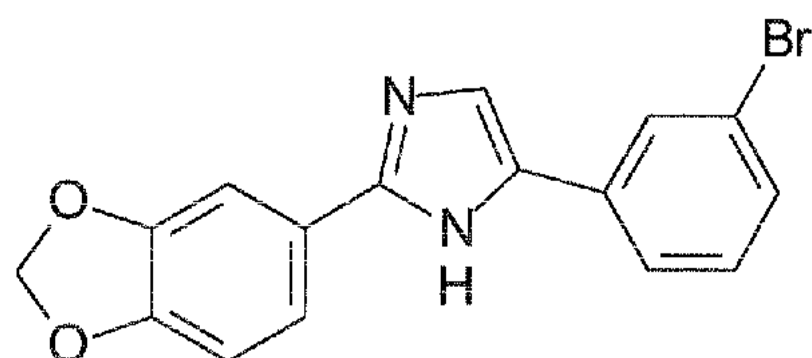
2-(1,3-benzodioxol-5-yl)-5-(3-bromophenyl)-1H-imidazole
