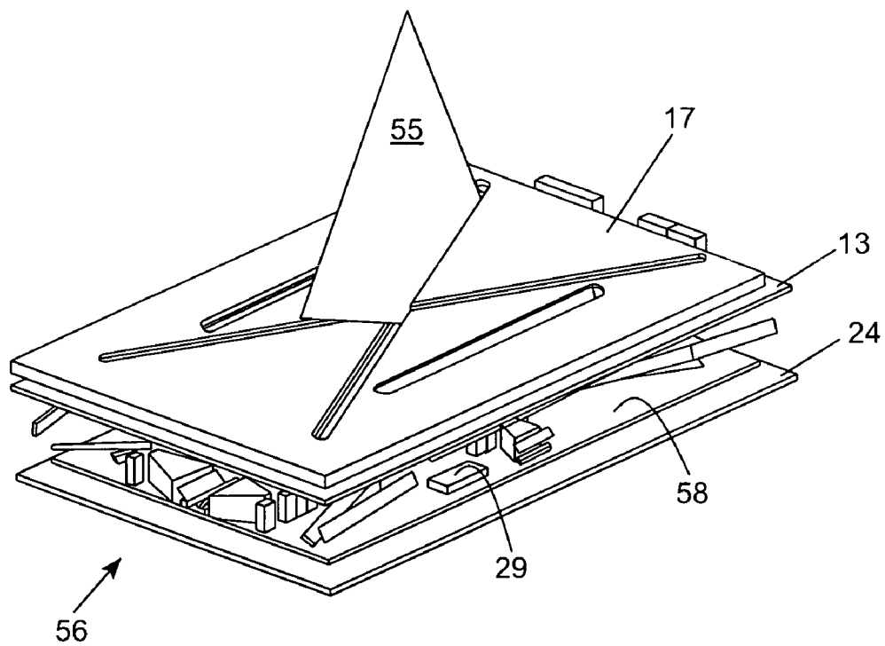
FIG. 3D
