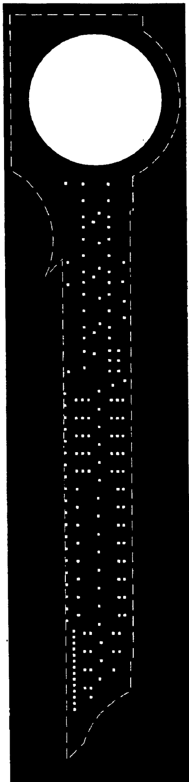
Contacts mask
