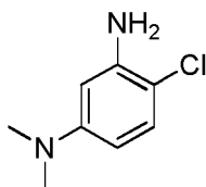
aniline 19
