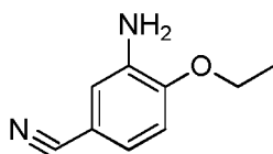
aniline 21
