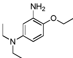
aniline 18
