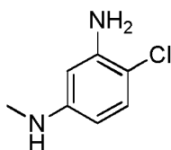
aniline 20
