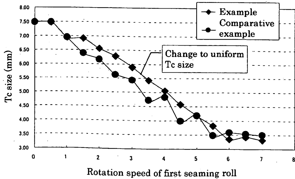
Fig. 17 Relationship between advancement of seaming process and change in Tc size
