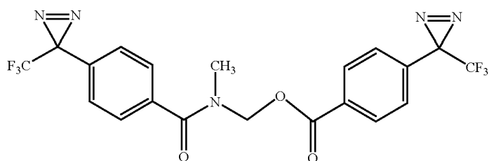
(N-methyl-4-(3-(trifluoromethyl)-3H-diazirin-3-yl)benzamido)methyl zoate; and
