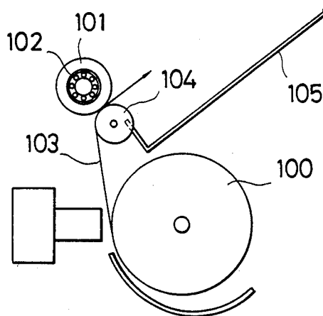
FIG. 7 PRIOR ART
