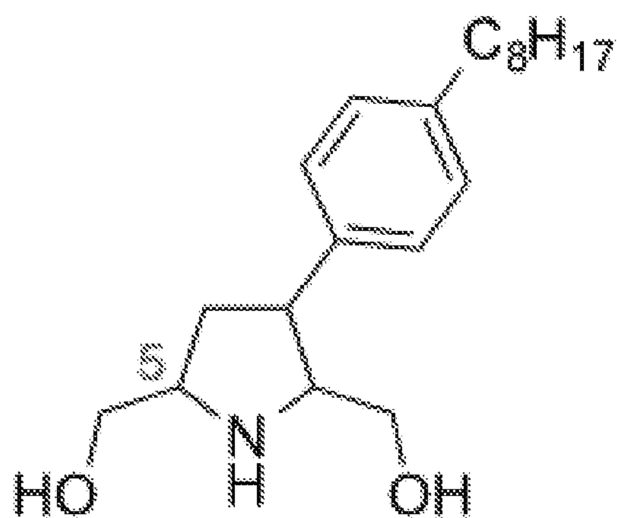
Generic constrained C-aryl analogue A
