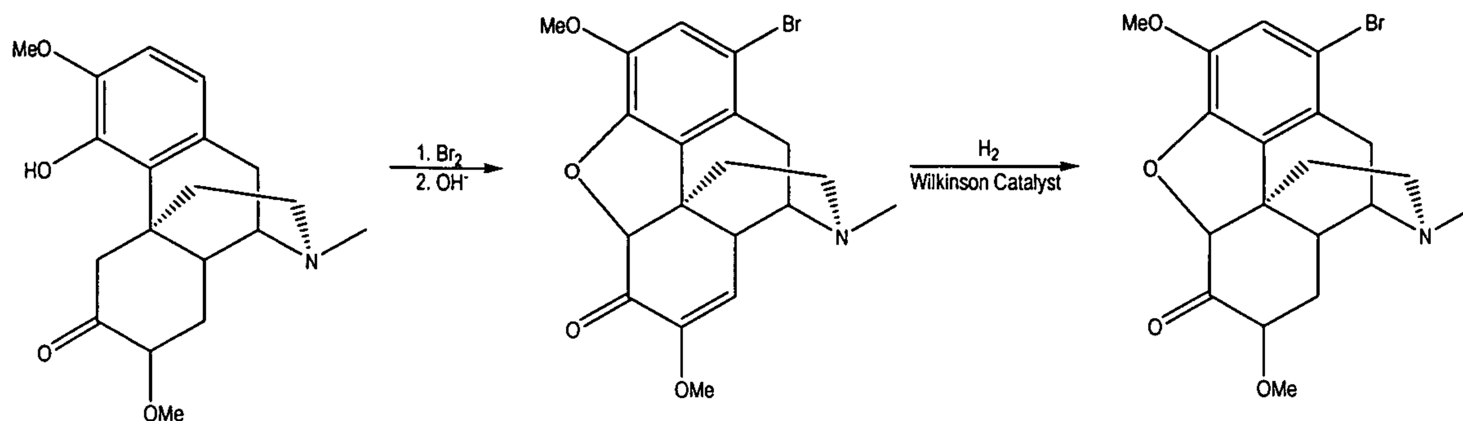
Reaction Scheme 5:
