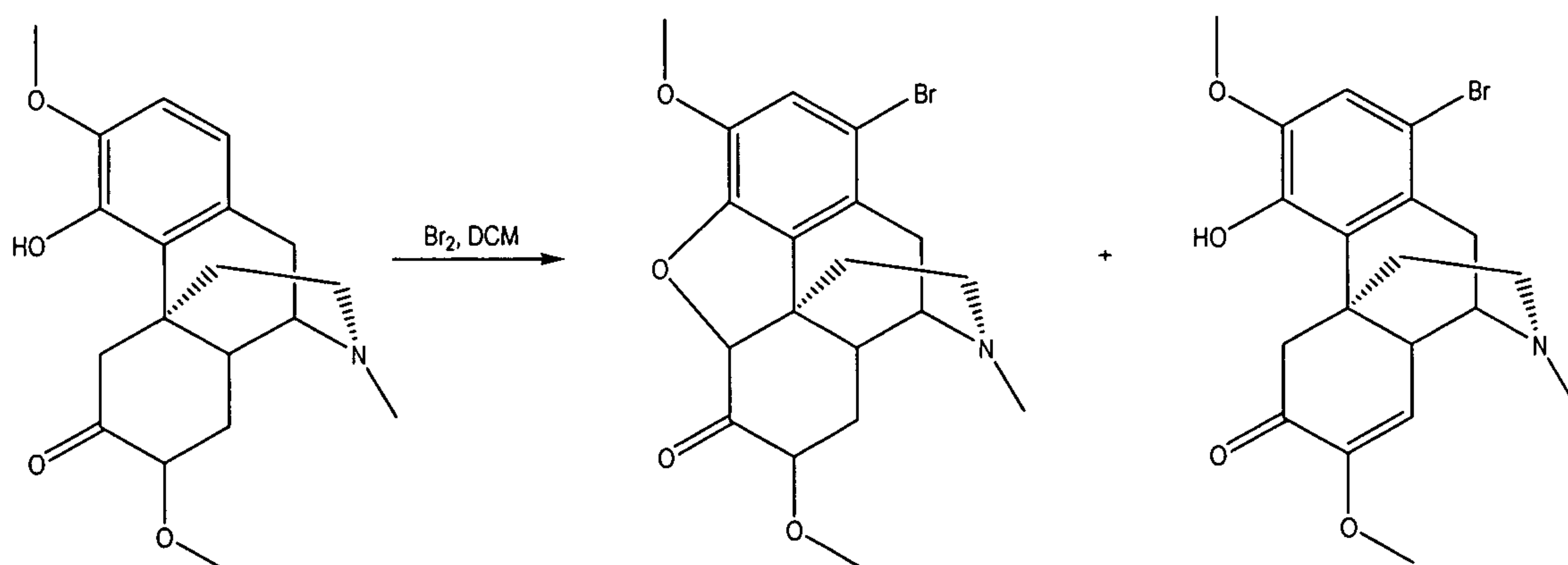
Reaction Scheme 3:
