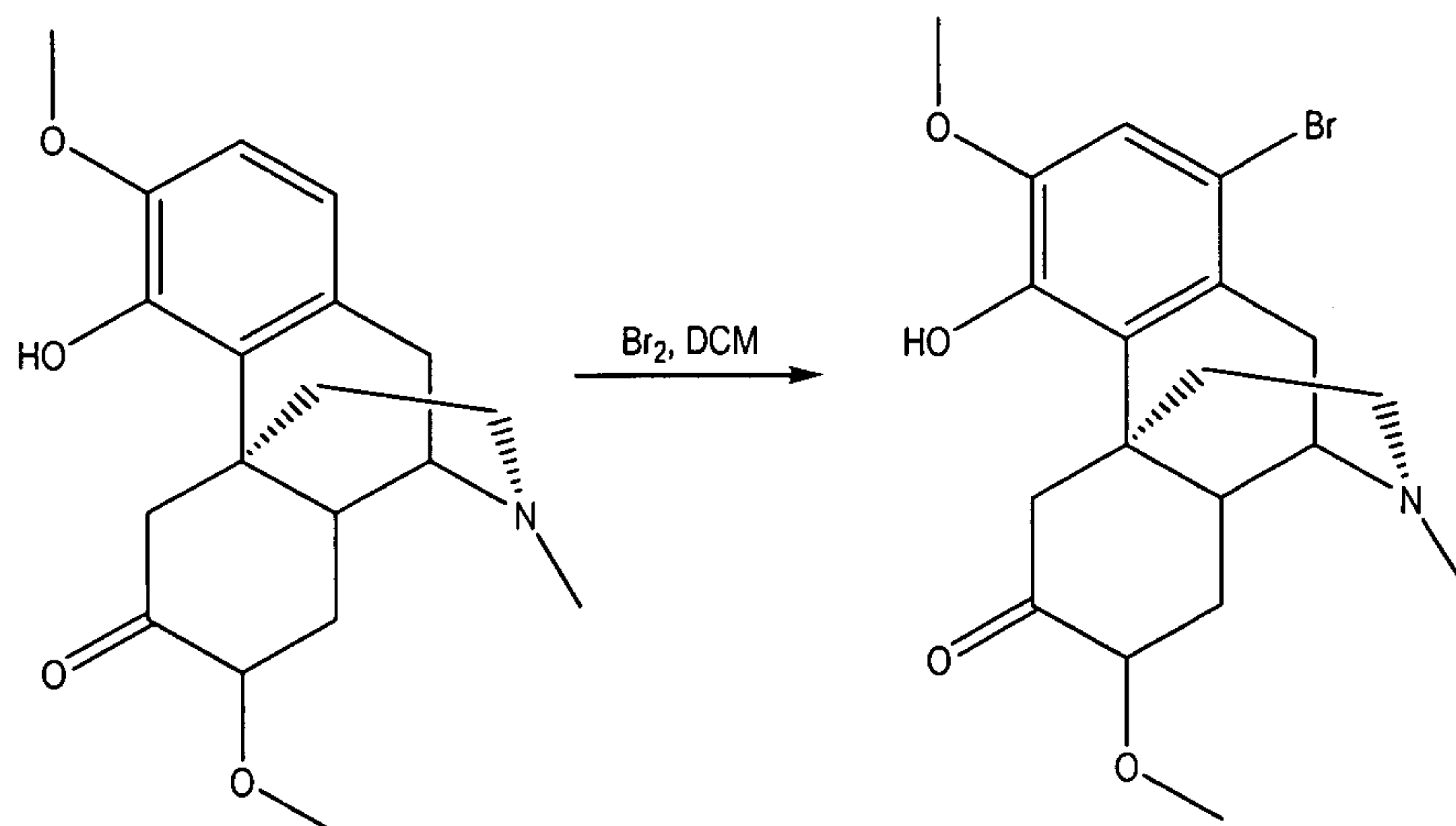
Reaction Scheme 4:
