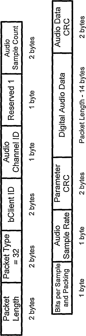
Audio Stream Packet
