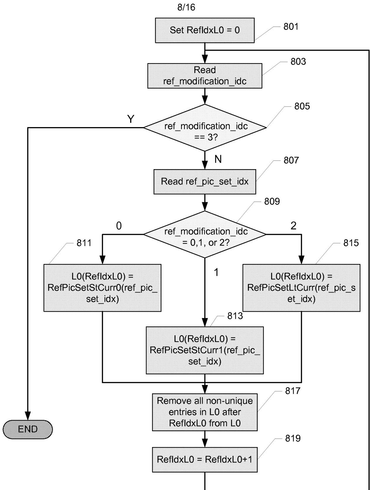
FIG. 8 (PRIOR ART)
