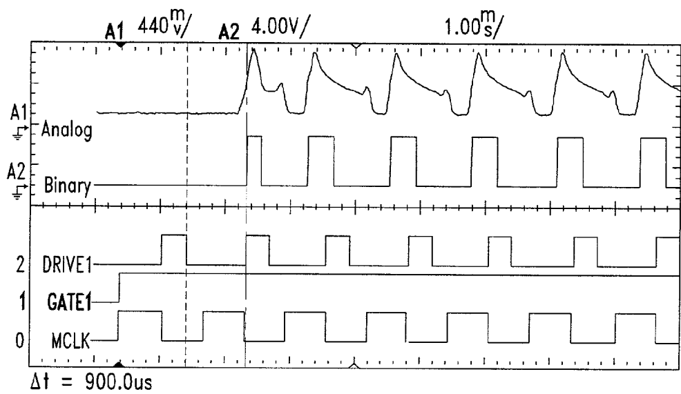
First Droplets of a Sweep Indicating Smaller First Droplet
