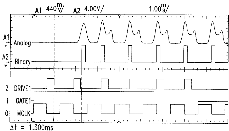
-BDD Output Signals for Premature First Droplet
