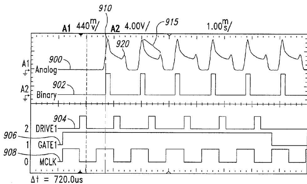
BDD Output Signals for Typical Droplet Formation
