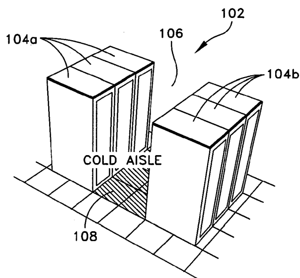
COLD-AISLE (RAISED-FLOOR) CLUSTER
