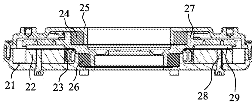
FIG. 2 (PRIOR ART)
