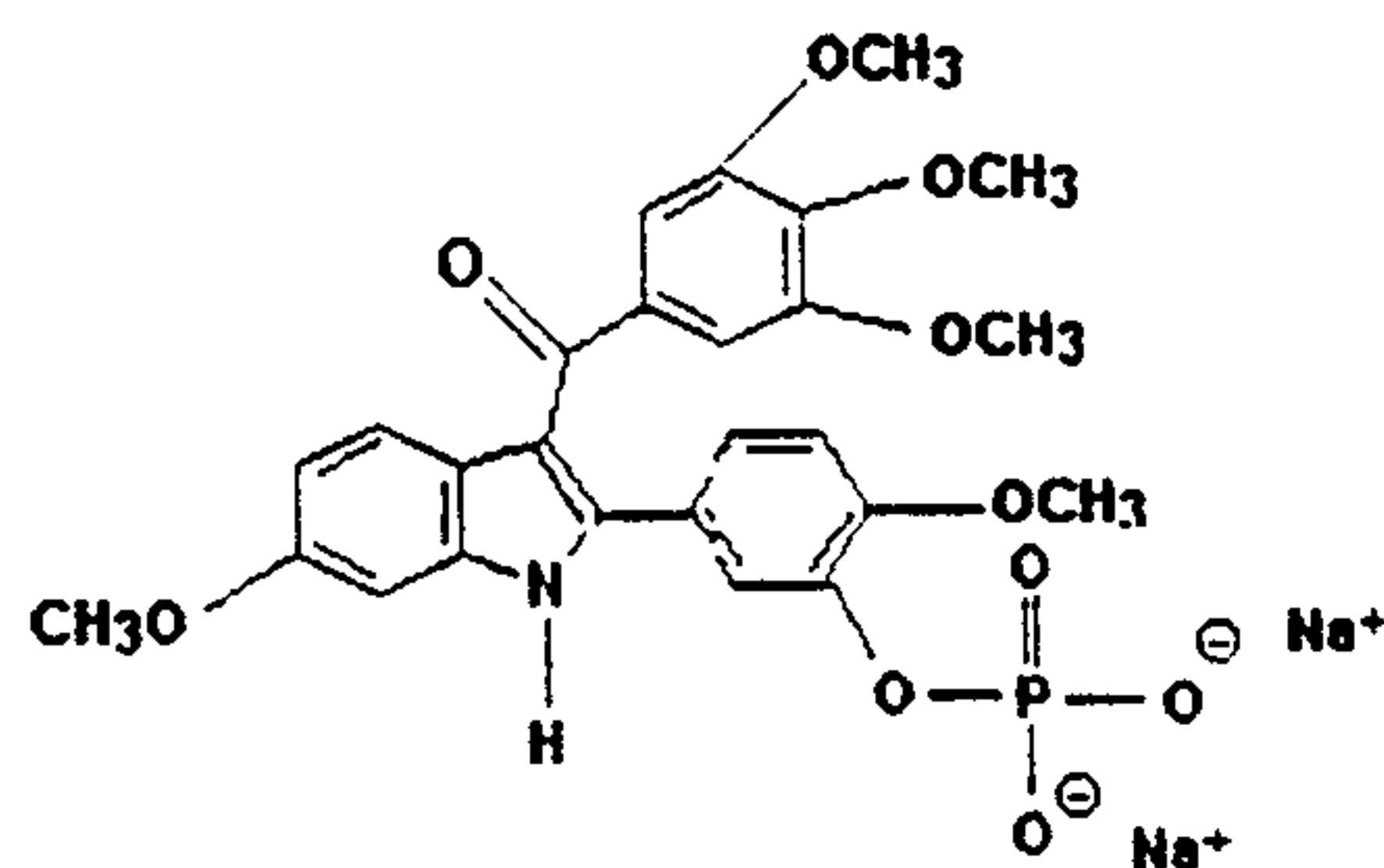
Indole sodium phosphate prodrug
