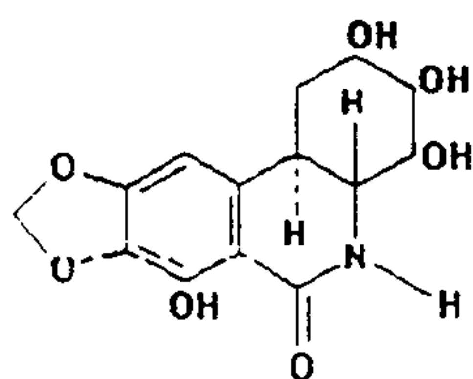
Pancratistatin
