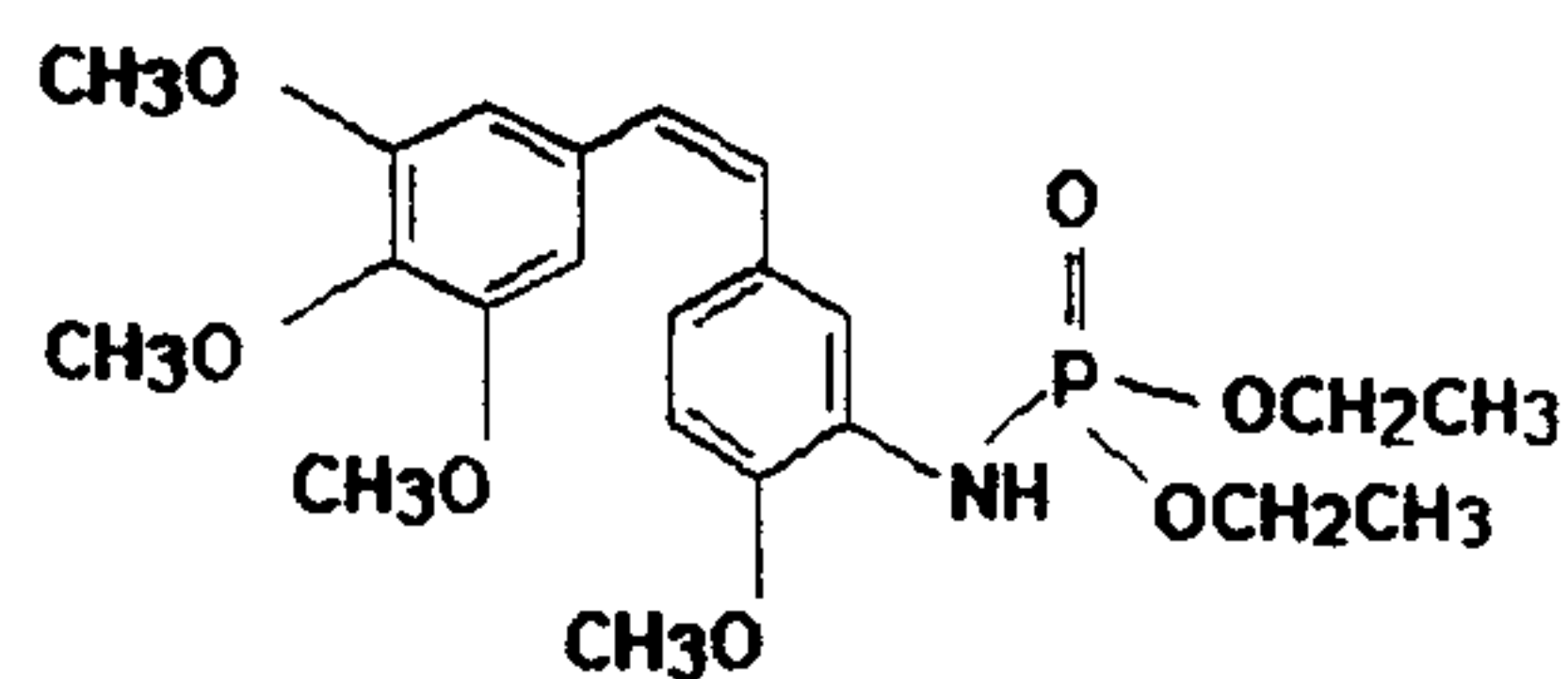
PM -VI -19C Amino Combretastatin A4 Phosphoro amidate prodrug
