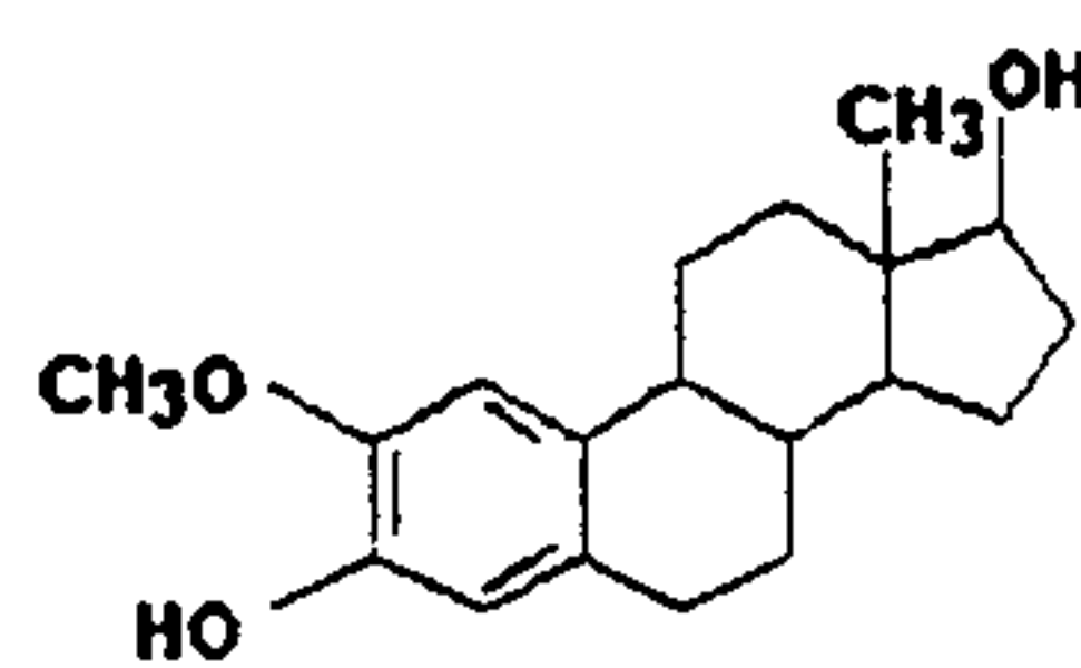
2-Methoxyestradiol
