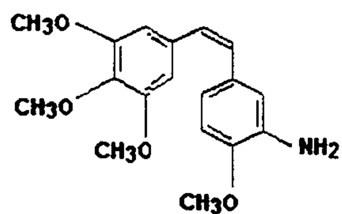
Amino Combretastatin A4 1-(3 amino -4 - methoxy phenyl) 2-(3,4,5 - tri methoxy phenyl) - ethene
