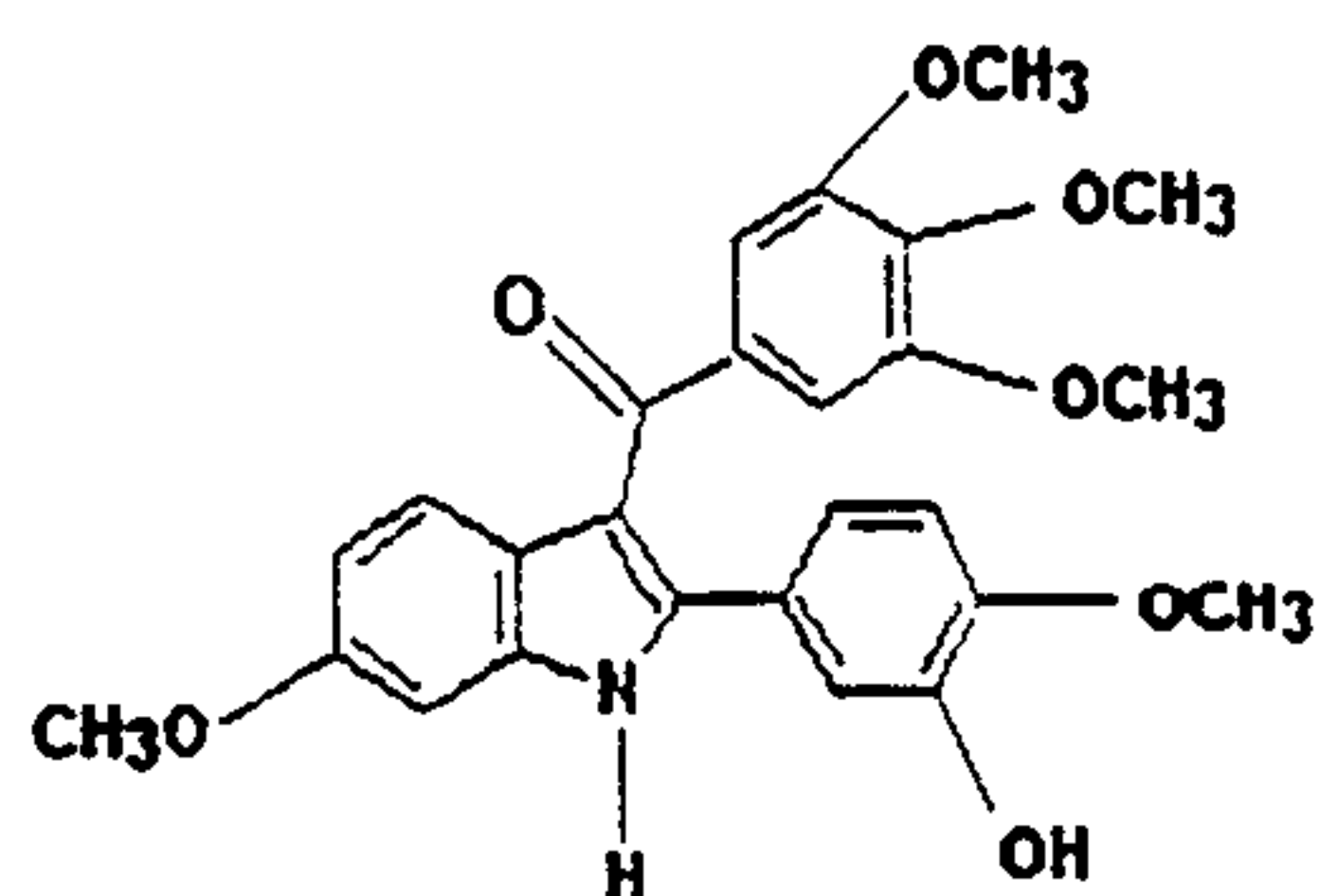
3 - (3',4',5' trimethoxy benzoyl) - 2- (4' - methoxy 5' - hydroxy phenyl)-6-methoxy indole
