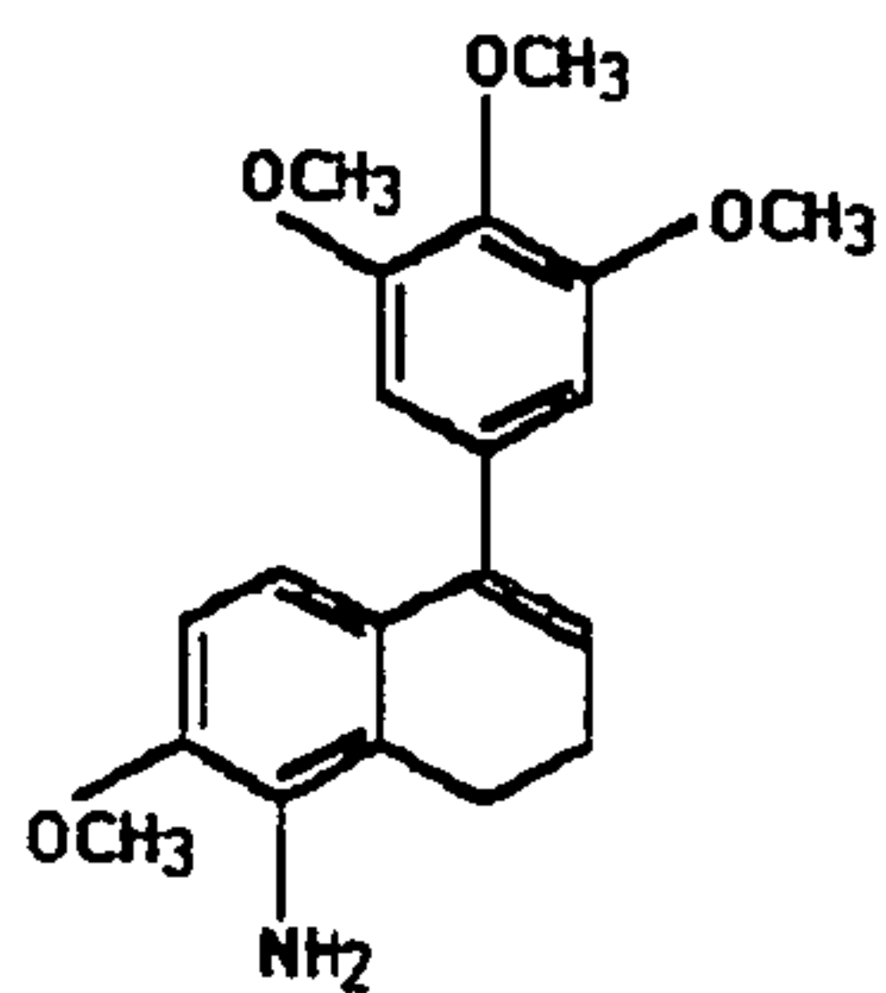
Amino dihydronaphthalene analog
