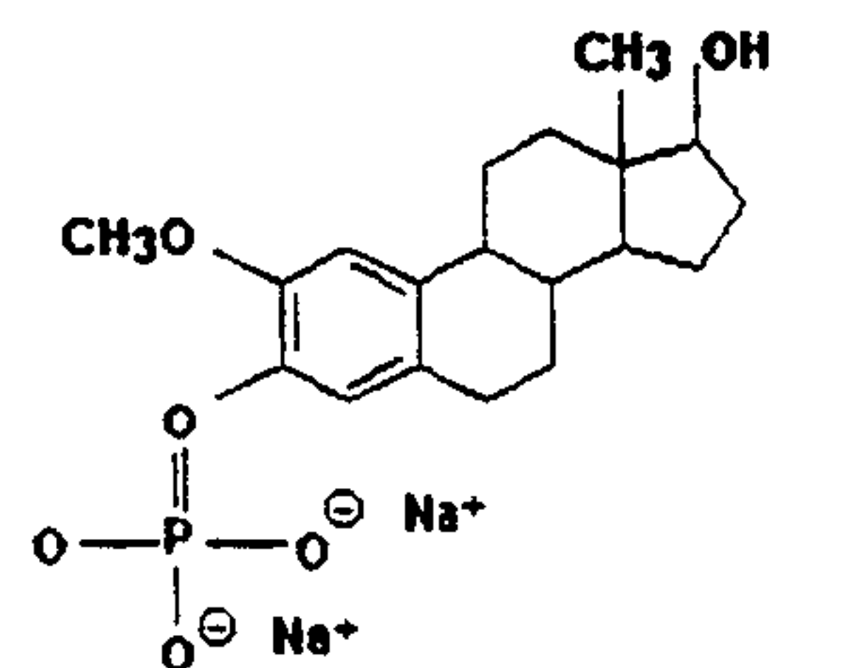
2-Methoxyestradiol sodium phosphate prodrug
