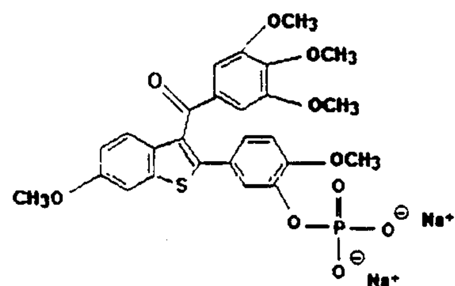
VPM-V-152 benzo(b)thiophene sodium phosphate prodrug
