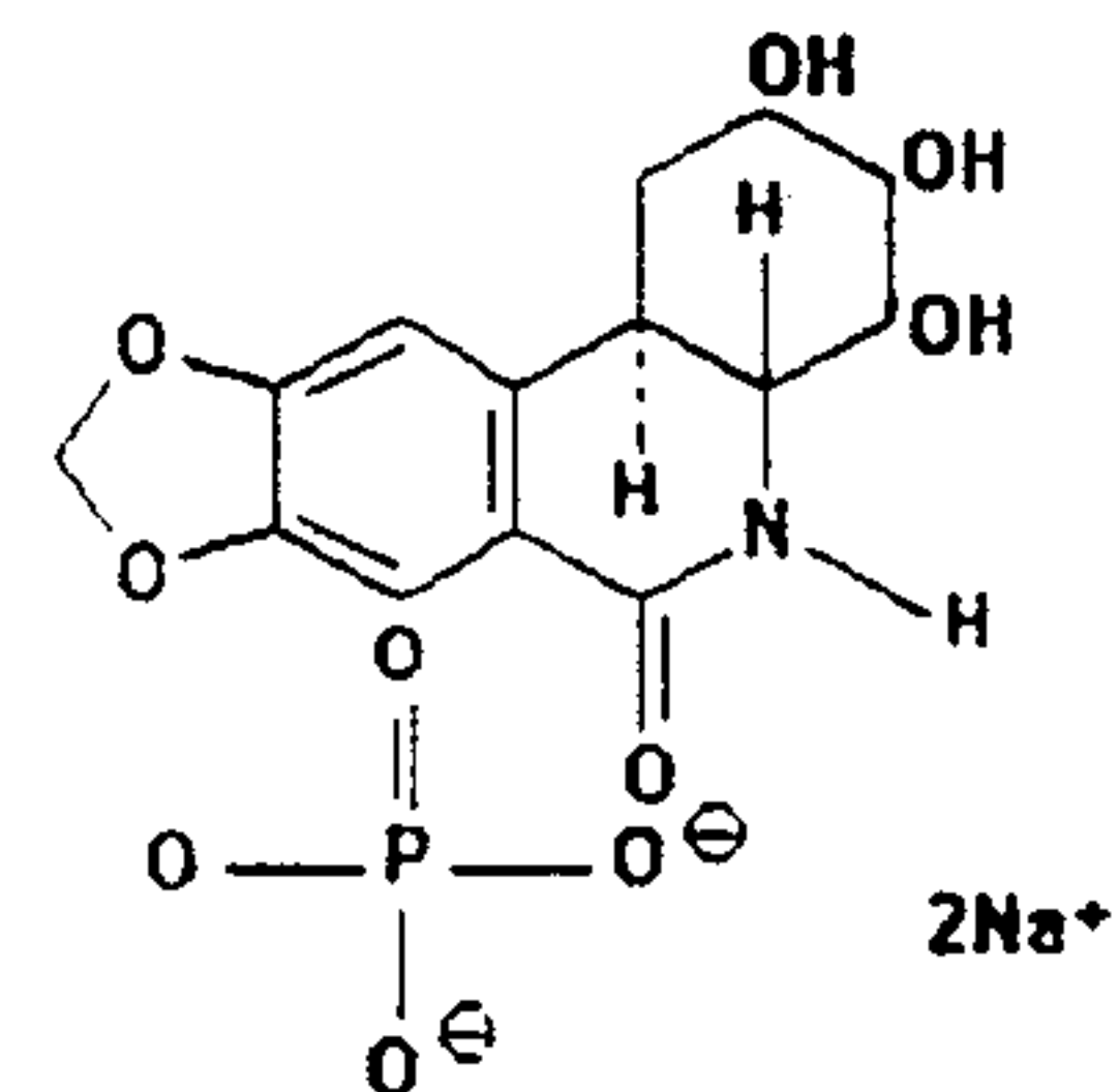
Pancratistatin sodium phosphate prodrug
