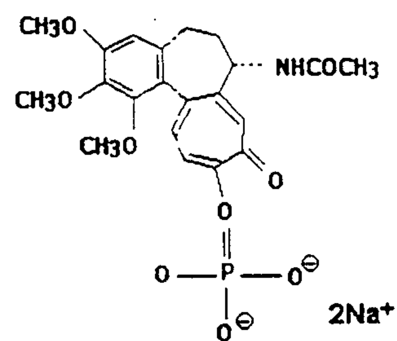
Colchicine sodium phosphate prodrug
