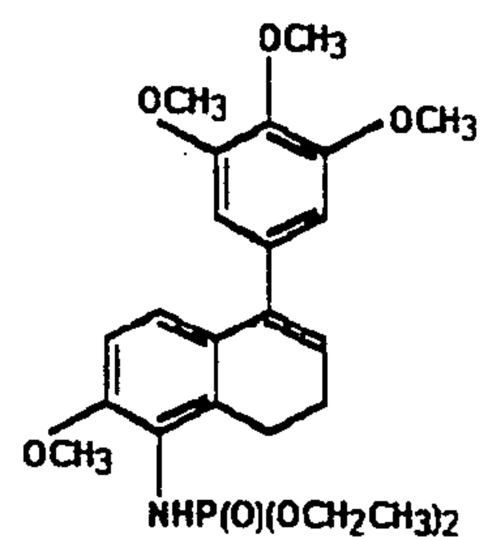
Amino dihydronaphthalene phosphoro amidate
