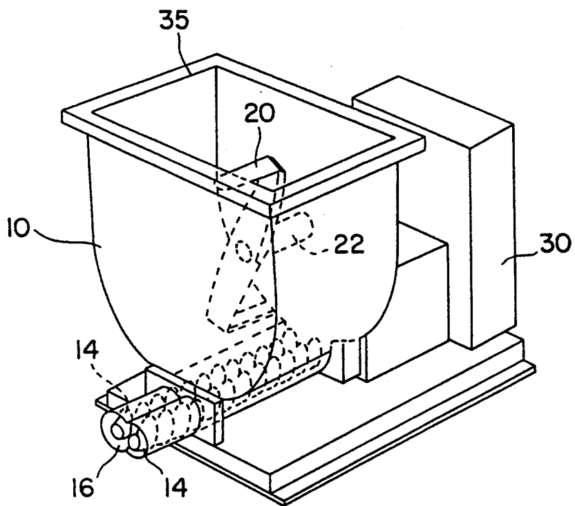
FIG. 1 PRIOR ART
