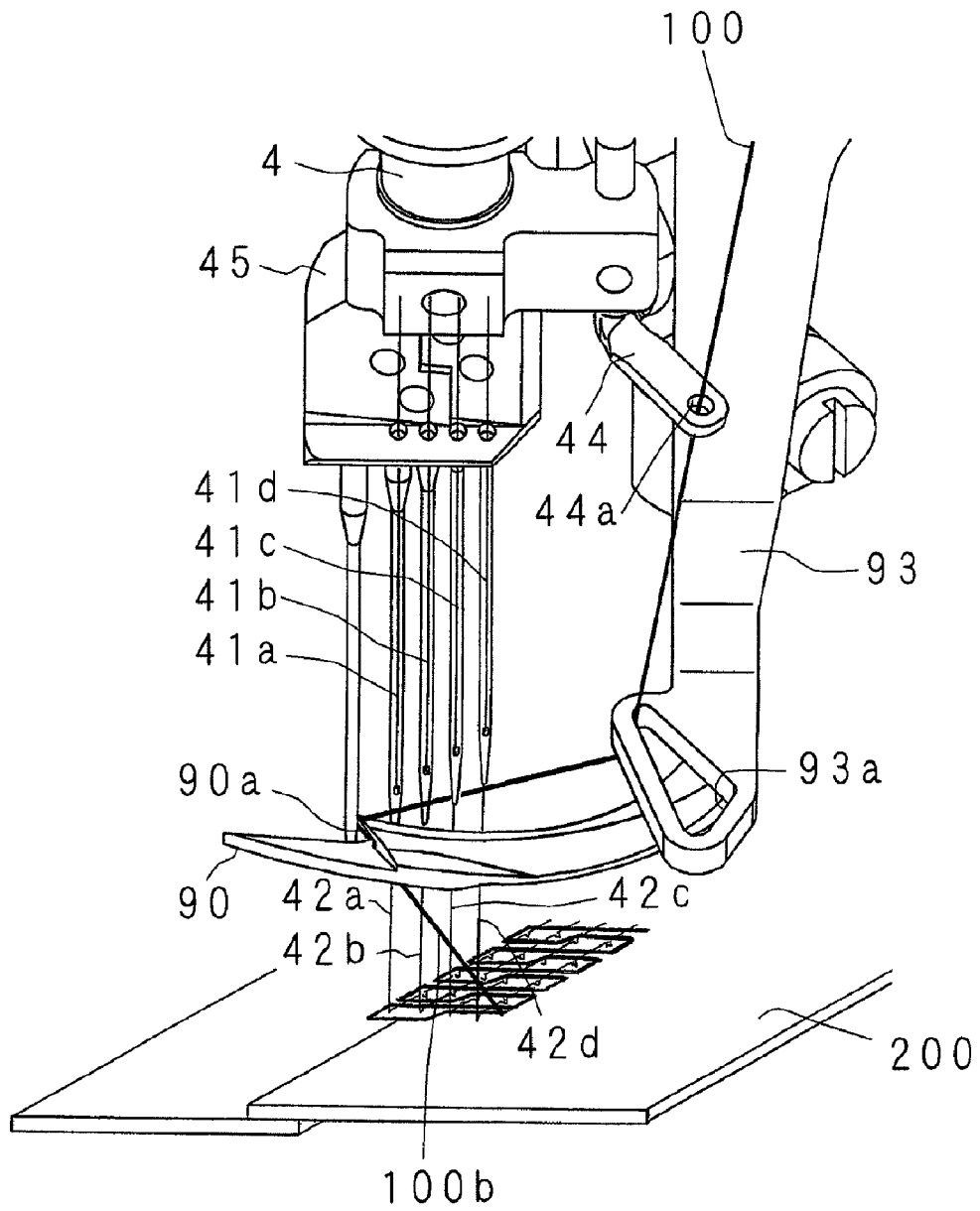
FIG. 1 PRIOR ART
