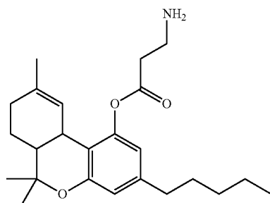
Chemical Formula: C_{24}H_{35}NO_3 Molecular Weight: 385.5396 THC-B-alanine (12)
