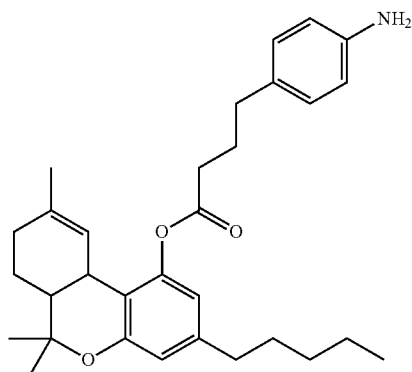
Chemical Formula: C_{31}H_{41}NO_3 Molecular Weight: 475.6621 THC-4-(4-amino-phenyl)butyrate (13)
