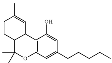
Structure of \Delta^9 -Tetrahydrocannabinol (THC)
