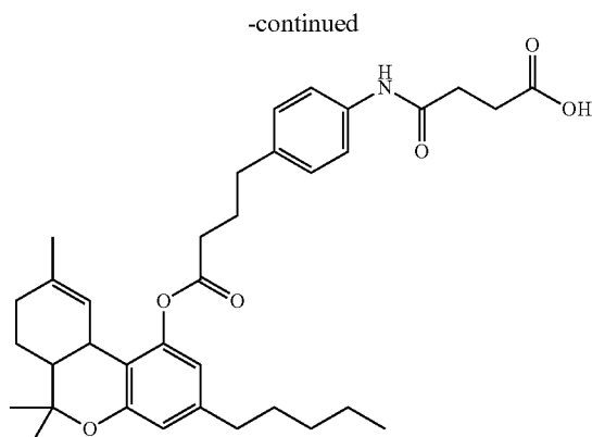
Chemical Formula: C_{35}H_{45}NO_6 Molecular Weight: 575.7349 THC-4-(4-amino-phenyl)butyrate hemisuccinate (14)
