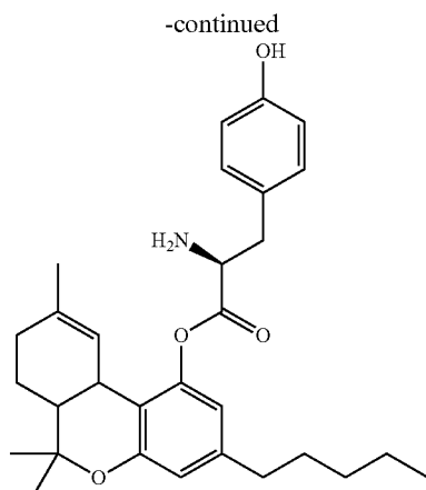
Chemical Formula: C_{30}H_{39}NO_4 Molecular Weight: 477.6350 THC-tyrosinate (11)
