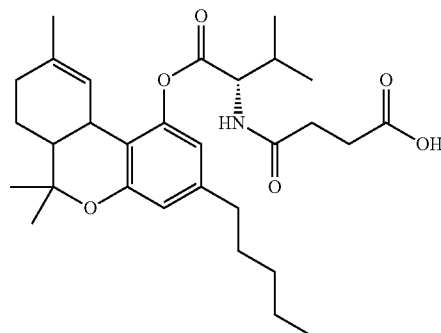
Chemical Formula: C_{30}H_{43}NO_6 Molecular Weight: 513.6655 THC-valinate-hemisuccinate (15)
