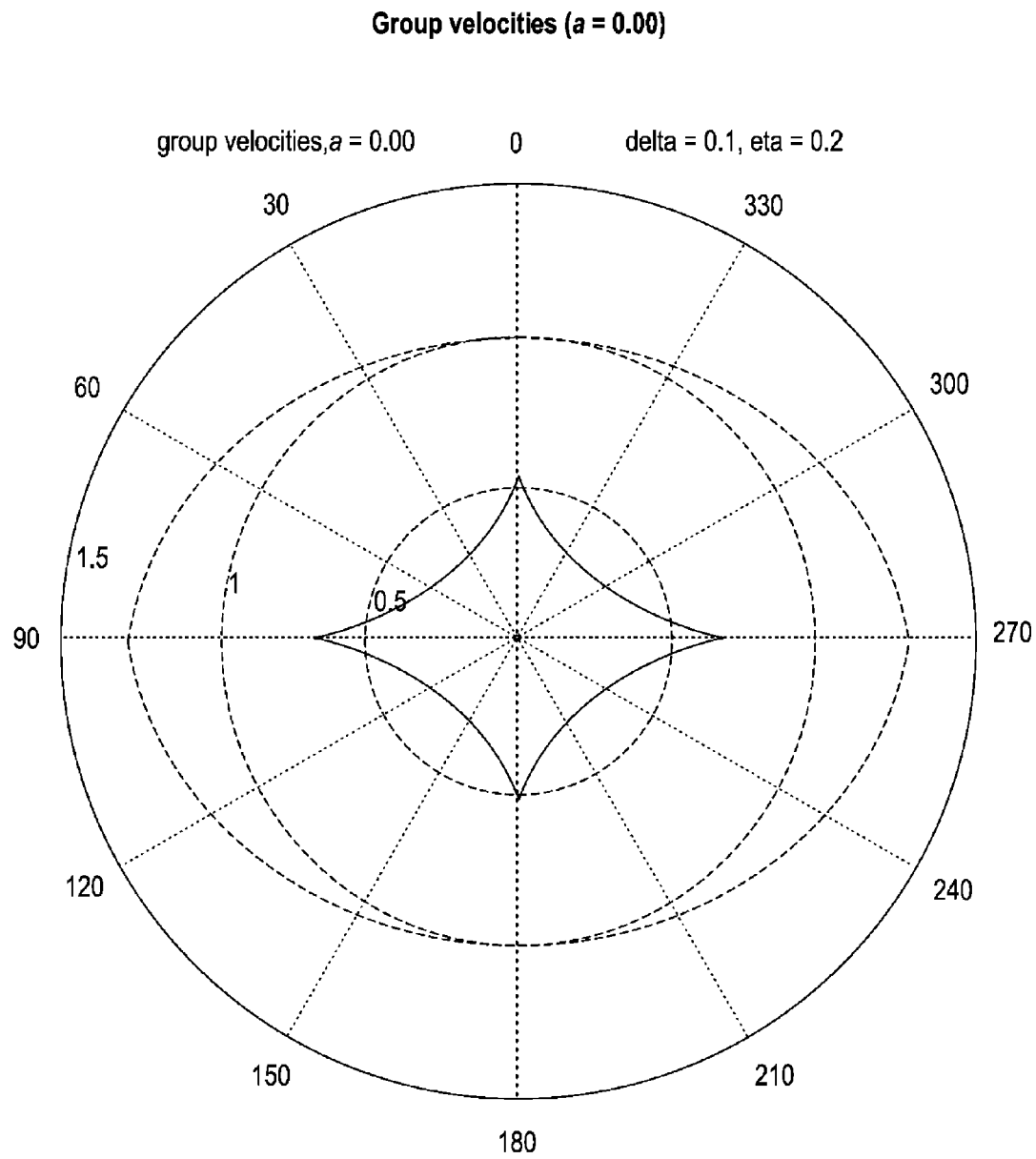
FIG. 9 (Prior Art)
