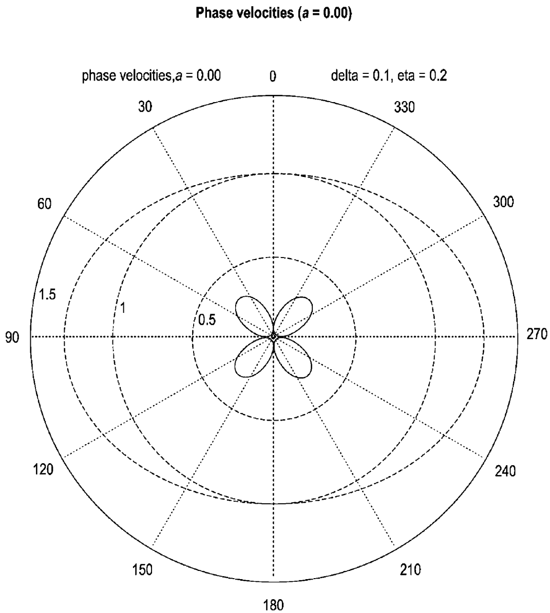
FIG. 8 (Prior Art)
