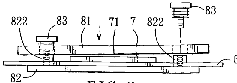
FIG. 2 PRIOR ART
