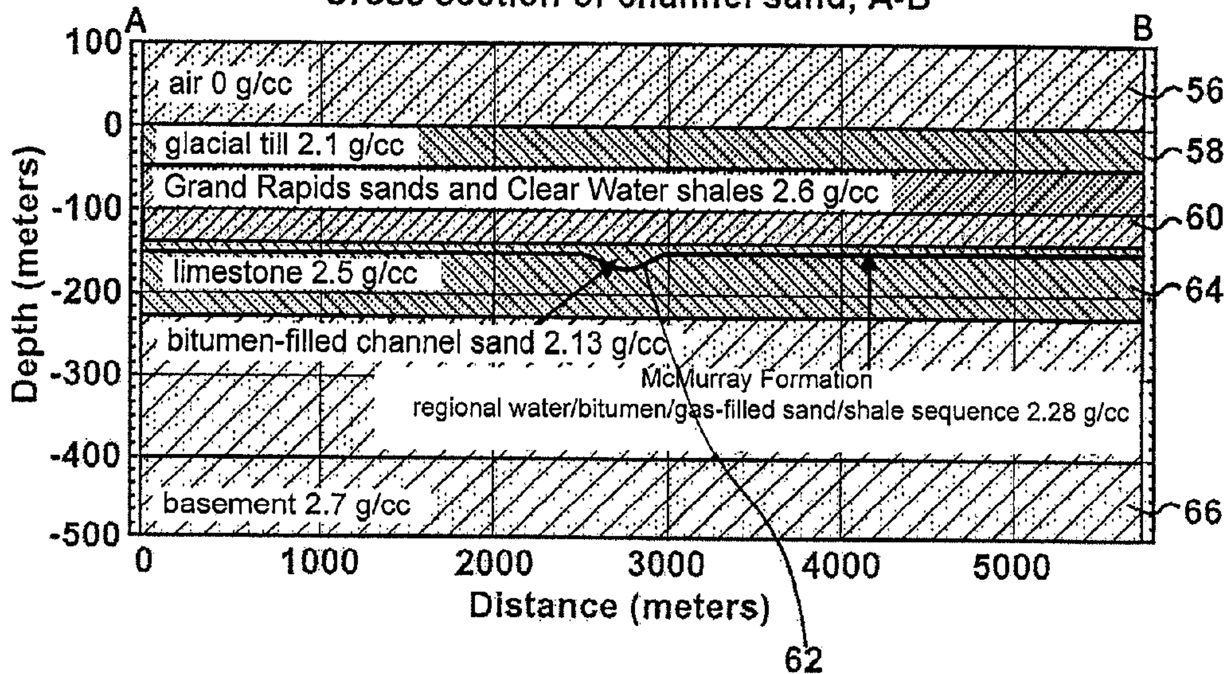
Cross section of channel sand, A-B
