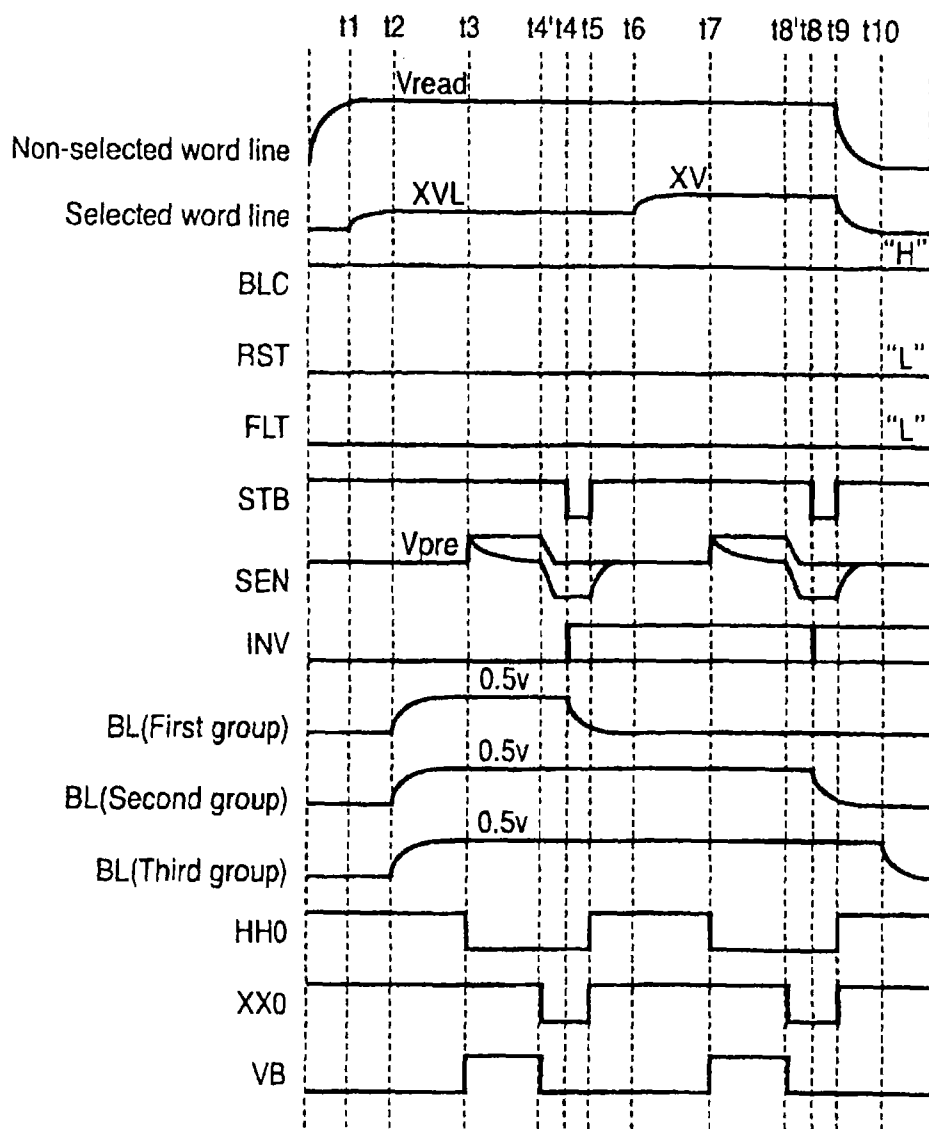
FIG. 11 PRIOR ART
