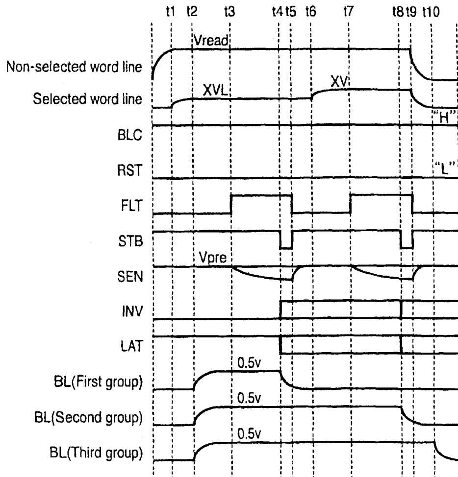
FIG. 9 PRIOR ART
