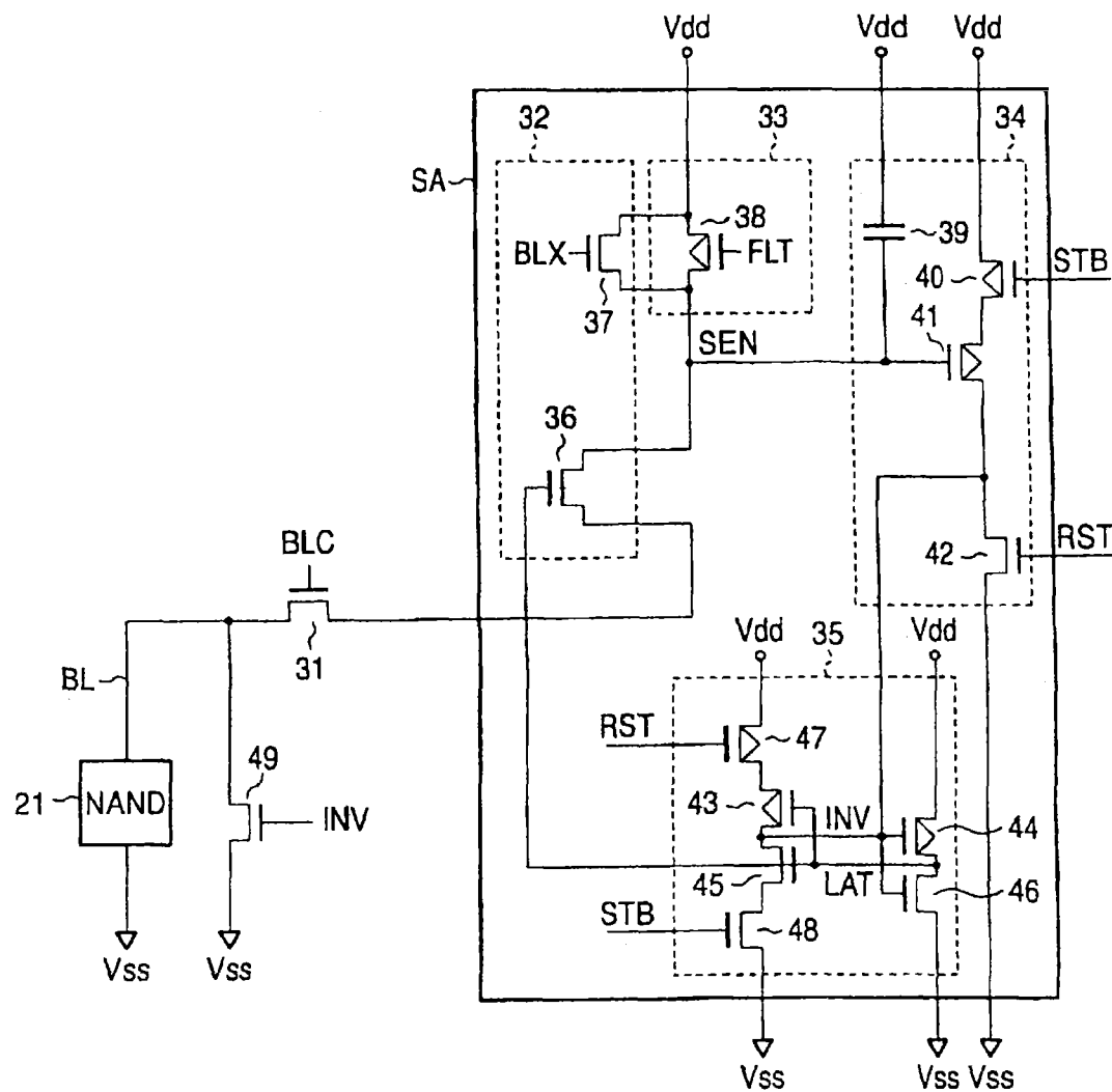
FIG. 8 PRIOR ART
