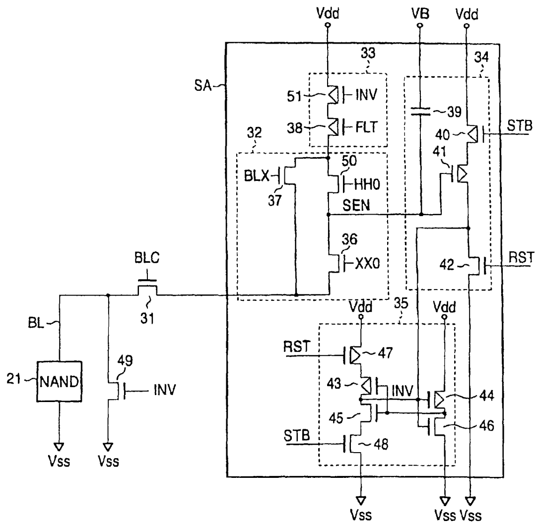
FIG. 10 PRIOR ART
