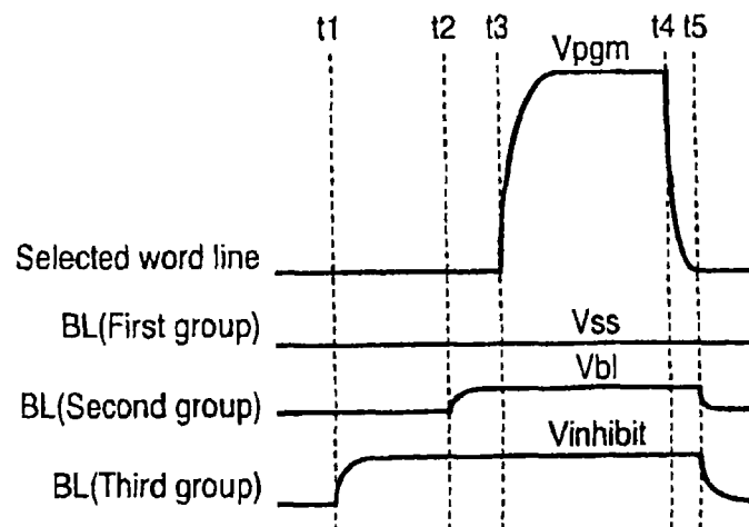
FIG. 12 PRIOR ART
