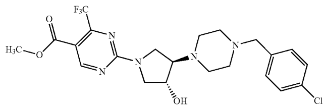
methyl 2-{3-[4-(4-chlorobenzyl)piperazin-1-yl]-4-hydroxypyrrolidin-1-yl}-4-(trifluoromethyl)pyrimidine-5-carboxylate
