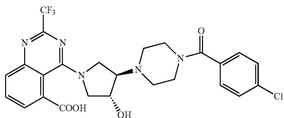
4-{3-[4-(4-chlorobenzoyl)piperazin-1-yl]-4-hydroxypyrrrolidin-1-yl}-2-(trifluoromethyl)quinazoline-5-carboxylic acid
