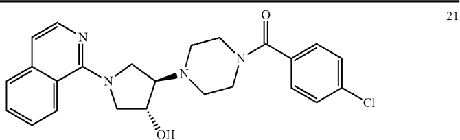
4-[4-(4-chlorobenzoyl)piperazin-1-yl]-1-isoquinolin-1-ylpyrrolidin-3-ol
