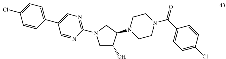
4-[4-(4-chlorobenzoyl)piperazin-1-yl]-1-[5-(4-chlorophenyl)pyrimidin-2-yl]pyrrolidin-3-ol
