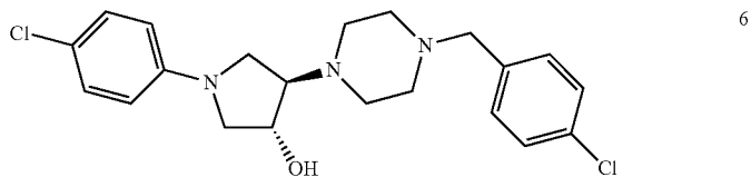
4-[4-(4-chlorobenzyl)piperazin-1-yl]-1-(4-chlorophenyl)pyrrolidin-3-ol
