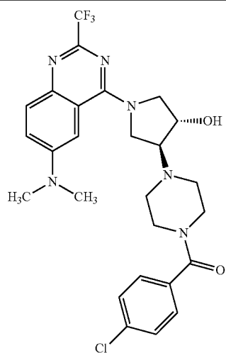
4-[4-(4-chlorobenzoyl)piperazin-1-yl]-1-[6-(dimethylamino)-2-(trifluoromethyl)quinazolin-4-yl]pyrrolidin-3-ol
