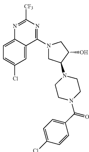
4-[4-(4-chlorobenzoyl)piperazin-1-yl]-1-[6-chloro-2-(trifluoromethyl)quinazolin-4-yl]pyrrolidin-3-ol
