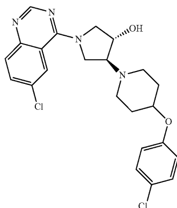
4-[4-(4-chlorophenoxy)piperidin-1-yl]-1-(6-chloroquinazolin-4-yl)pyrrolidin-3-ol
