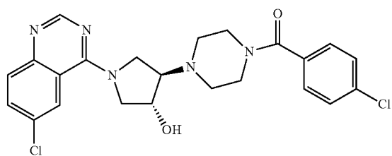
4-[4-(4-chlorobenzoyl)piperazin-1-yl]-1-(6-chloroquinazolin-4-yl)pyrrolidin-3-ol
