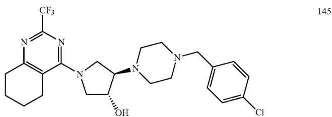
4-[4-(4-chlorobenzyl)piperazin-1-yl]-1-[2-(trifluoromethyl)-5,6,7,8-tetrahydroquinazolin-4-yl]pyrrolidin-3-ol
