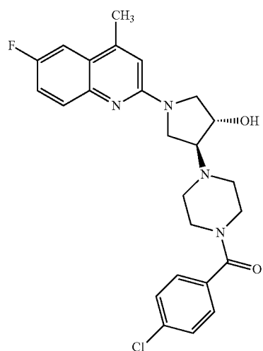
4-[4-(4-chlorobenzoyl)piperazin-1-yl]-1-(6-fluoro-4-methylquinolin-2-yl)pyrrolidin-3-ol
