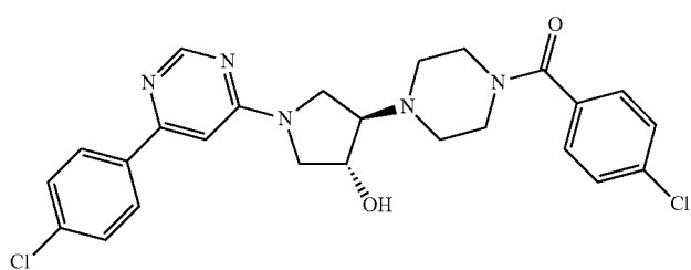
4-[4-(4-chlorobenzoyl)piperazin-1-yl]-1-[6-(4-chlorophenyl)pyrimidin-4-yl]pyrrolidin-3-ol
