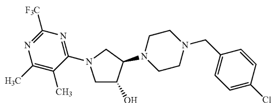
4-[4-(4-chlorobenzyl)piperazin-1-yl]-1-(5,6-dimethyl-2-(trifluoromethyl)pyrimidin-4-yl)pyrrolidin-3-ol
