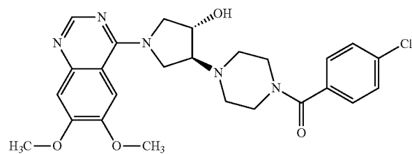
4-[4-(4-chlorobenzoyl)piperazin-1-yl]-1-(6,7-dimethoxyquinazolin-4-yl)pyrrolidin-3-ol
