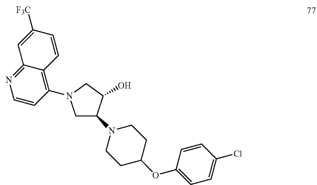
4-[4-(4-chlorophenoxy)piperidin-1-yl]-1-[7-(trifluoromethyl)quinolin-4-yl]pyrrolidin-3-ol
