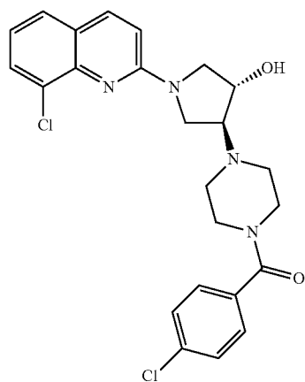
4-[4-(4-chlorobenzoyl)piperazin-1-yl]-1-(8-chloroquinolin-2-yl)pyrrolidin-3-ol
