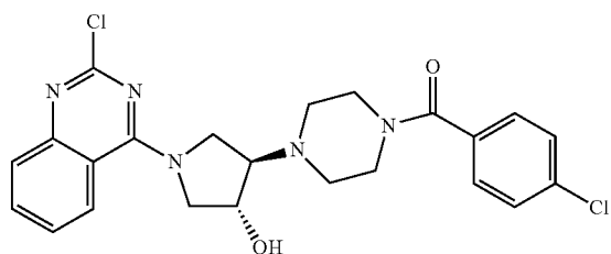
4-[4-(4-chlorobenzoyl)piperazin-1-yl]-1-(2-chloroquinazolin-4-yl)pyrrolidin-3-ol
