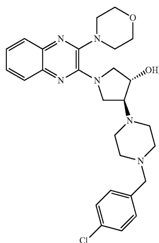
4-[4-(4-chlorobenzyl)piperazin-1-yl]-1-(3-morpholin-4-ylquinoxalin-2-yl)pyrrolidin-3-ol
