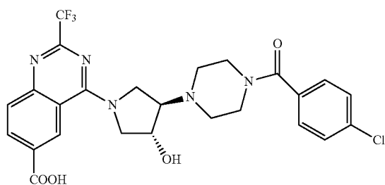
4-[(3R,4R)-3-[4-(4-chlorobenzoyl)piperazin-1-yl]-4-hydroxypyrrolidin-1-yl]-2-(trifluoromethyl)quinazoline-6-carboxylic acid
