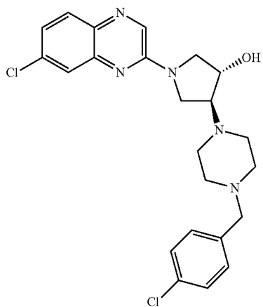
4-[4-(4-chlorobenzyl)piperazin-1-yl]-1-(7-chloroquinoxalin-2-yl)pyrrolidin-3-ol
