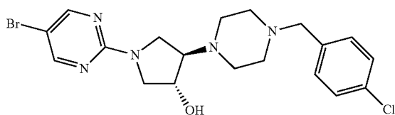
1-(5-bromopyrimidin-2-yl)-4-[4-(4-chlorobenzyl)piperazin-1-yl]pyrrolidin-3-ol
