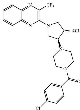
4-[4-(4-chlorobenzoyl)piperazin-1-yl]-1-[3-(trifluoromethyl)quinoxalin-2-yl]pyrrolidin-3-ol
