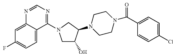
4-[4-(4-chlorobenzoyl)piperazin-1-yl]-1-(7-fluoroquinazolin-4-yl)pyrrolidin-3-ol
