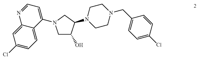
4-[4-(4-chlorobenzyl)piperazin-1-yl]-1-(7-chloroquinolin-4-yl)pyrrolidin-3-ol
