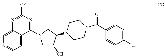
4-[4-(4-chlorobenzoyl)piperazin-1-yl]-1-[2-(trifluoromethyl)pyrido[3,4-d]pyrimidin-4-yl]pyrrolidin-3-ol
