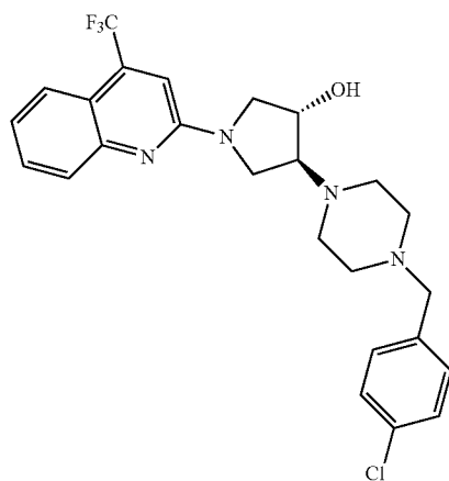
4-[4-(4-chlorobenzyl)piperazin-1-yl]-1-[4-(trifluoromethyl)quinolin-2-yl]pyrrolidin-3-ol
