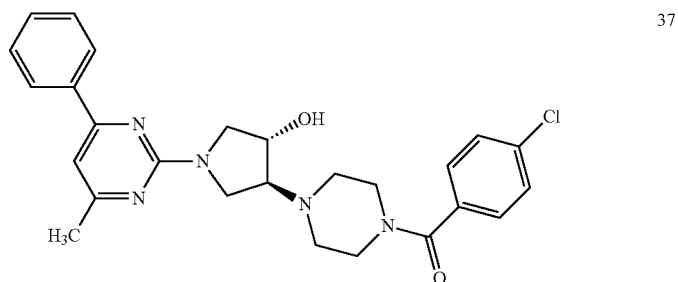
4-[4-(4-chlorobenzoyl)piperazin-1-yl]-1-(4-methyl-6-phenylpyrimidin-2-yl)pyrrolidin-3-ol
