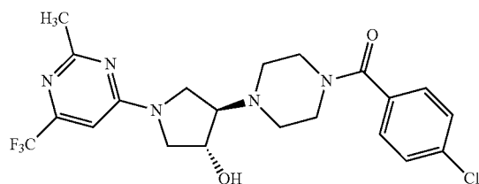
4-[4-(4-chlorobenzoyl)piperazin-1-yl]-1-[2-methyl-6-(trifluoromethyl)pyrimidin-4-yl]pyrrolidin-3-ol
