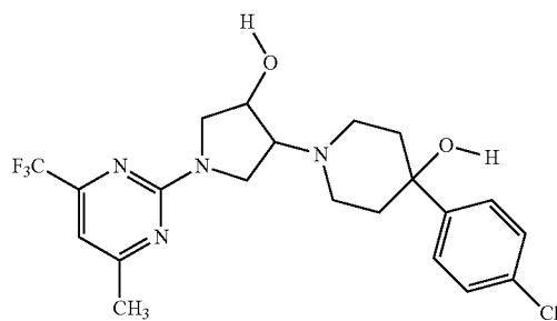
4-(4-chlorophenyl)-1-{4-hydroxy-1-[4-methyl-6-(trifluoromethyl)pyrimidin-2-yl]pyrrolidin-3-yl}piperidin-4-ol
