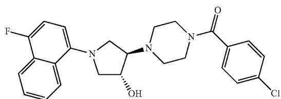
4-[4-(4-chlorobenzoyl)piperazin-1-yl]-1-(4-fluoro-1-naphthyl)pyrrolidin-3-ol
