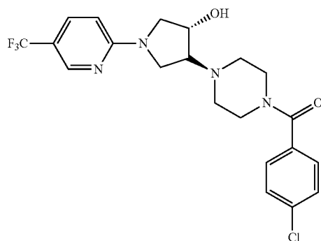
4-[4-(4-chlorobenzoyl)piperazin-1-yl]-1-[5-(trifluoromethyl)pyridin-2-yl]pyrrolidin-3-ol
