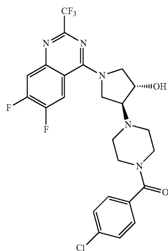
4-[4-(4-chlorobenzoyl)piperazin-1-yl]-1-[6,7-difluoro-2-(trifluoromethyl)quinazolin-4-yl]pyrrolidin-3-ol
