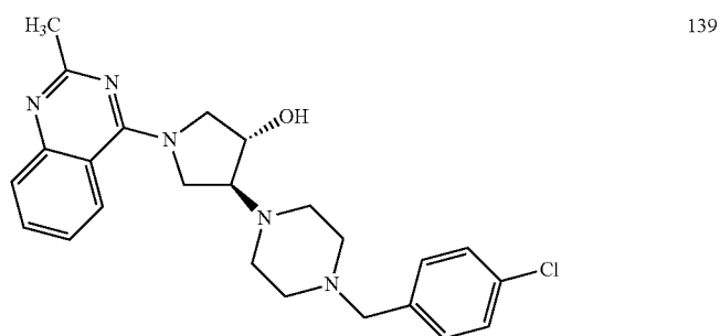
4-[4-(4-chlorobenzyl)piperazin-1-yl]-1-(2-methylquinazolin-4-yl)pyrrolidin-3-ol
