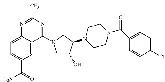
4-((3R,4R)-3-[4-(4-chlorobenzoyl)piperazin-1-yl]-4-hydroxypyrrolidin-1-yl)-2-(trifluoromethyl)quinazoline-6-carboxamide
