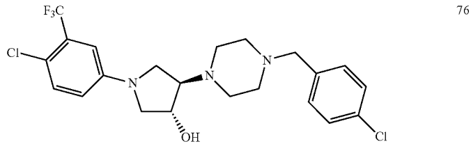
4-[4-(4-chlorobenzyl)piperazin-1-yl]-1-[4-chloro-3-(trifluoromethyl)phenyl]pyrrolidin-3-ol
