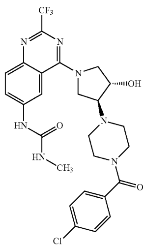
N-[4-((3S,4S)-3-[4-(4-chlorobenzoyl)piperazin-1-yl]-4-hydroxypyrrolidin-1-yl)-2-(trifluoromethyl)quinazolin-6-yl]-N'-methylurea
