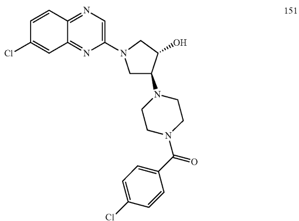
(3S,4S)-4-[4-(4-chlorobenzoyl)piperazin-1-yl]-1-(7-chloroquinoxalin-2-yl)pyrrolidin-3-ol
