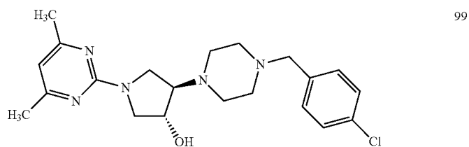
4-[4-(4-chlorobenzyl)piperazin-1-yl]-1-(4,6-dimethylpyrimidin-2-yl)pyrrolidin-3-ol
