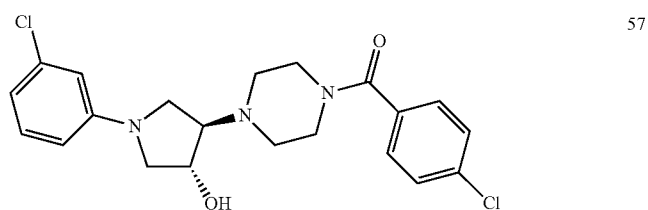
4-[4-(4-chlorobenzoyl)piperazin-1-yl]-1-(3-chlorophenyl)pyrrolidin-3-ol
