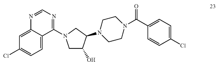
4-[4-(4-chlorobenzoyl)piperazin-1-yl]-1-(7-chloroquinazolin-4-yl)pyrrolidin-3-ol
