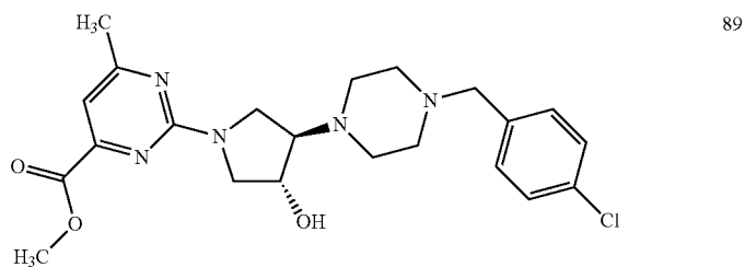
methyl 2-{3-[4-(4-chlorobenzyl)piperazin-1-yl]-4-hydroxypyrrolidin-1-yl}-6-methylpyrimidine-4-carboxylate
