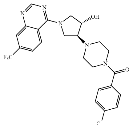
4-[4-(4-chlorobenzoyl)piperazin-1-yl]-1-[7-(trifluoromethyl)quinazolin-4-yl]pyrrolidin-3-ol
