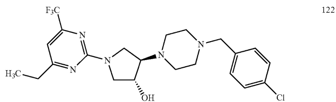
4-[4-(4-chlorobenzyl)piperazin-1-yl]-1-[4-ethyl-6-(trifluoromethyl)pyrimidin-2-yl]pyrrolidin-3-ol
