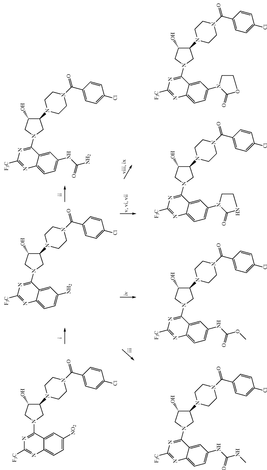
Scheme 9
