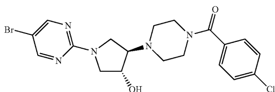
1-(5-bromopyrimidin-2-yl)-4-[4-(4-chlorobenzoyl)piperazin-1-yl]pyrrolidin-3-ol
