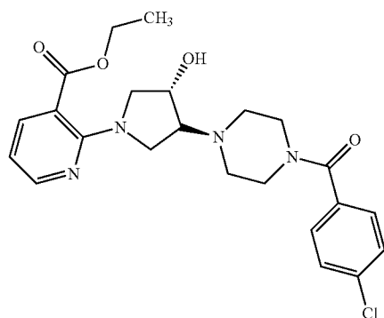
ethyl 2-(3-[4-(4-chlorobenzoyl)piperazin-1-yl]-4-hydroxypyrrolidin-1-yl)nicotinate
