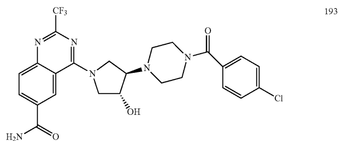
4-((3R,4R)-3-[4-(4-chlorobenzoyl)piperazin-1-yl]-4-hydroxypyrrolidin-1-yl)-2-(trifluoromethyl)quinazoline-6-carboxamide
