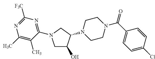
(3S,4S)-4-[4-(4-chlorobenzoyl)piperazin-1-yl]-1-[5,6-dimethyl-2-(trifluoromethyl)pyrimidin-4-yl]pyrrolidin-3-ol
