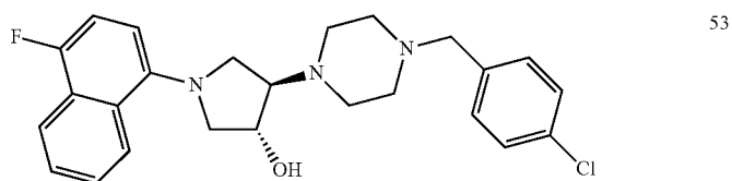
4-[4-(4-chlorobenzyl)piperazin-1-yl]-1-(4-fluoro-1-naphthyl)pyrrolidin-3-ol
