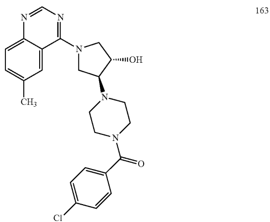
4-[4-(4-chlorobenzoyl)piperazin-1-yl]-1-(6-methylquinazolin-4-yl)pyrrolidin-3-ol
