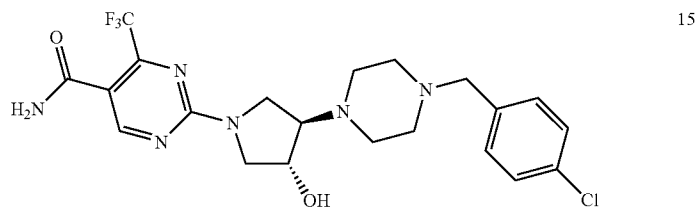
2-{3-[4-(4-chlorobenzoyl)piperazin-1-yl]-4-hydroxypyrrolidin-1-yl}-4-(trifluoromethyl)pyrimidine-5-carboxamide
