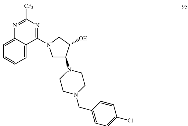
4-[4-(4-chlorobenzyl)piperazin-1-yl]-1-[2-(trifluoromethyl)quinazolin-4-yl]pyrrolidin-3-ol
