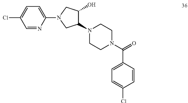
4-[4-(4-chlorobenzoyl)piperazin-1-yl]-1-(5-chloropyridin-2-yl)pyrrolidin-3-ol
