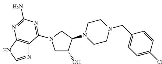
1-(2-amino-9H-purin-6-yl)-4-[4-(4-chlorobenzyl)piperazin-1-yl]pyrrolidin-3-ol
