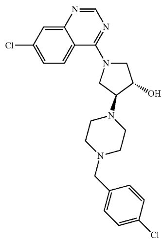
4-[4-(4-chlorobenzyl)piperazin-1-yl]-1-(7-chloroquinazolin-4-yl)pyrrolidin-3-ol
