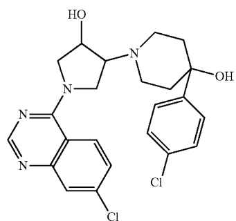
4-(4-chlorophenyl)-1-[1-(7-chloroquinazolin-4-yl)-4-hydroxypyrrolidin-3-yl]piperidin-4-ol
