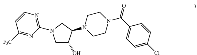
4-[4-(4-chlorobenzoyl)piperazin-1-yl]-1-[4-(trifluoromethyl)pyrimidin-2-yl]pyrrolidin-3-ol
