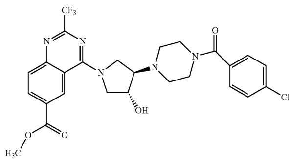
methyl 4-{3-[4-(4-chlorobenzoyl)piperazin-1-yl]-4-hydroxypyrrolidin-1-yl}-2-(trifluoromethyl)quinazoline-6-carboxylate
