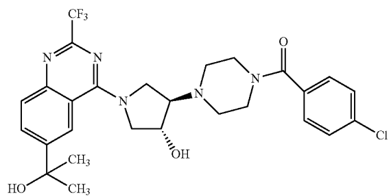
4-[4-(4-chlorobenzoyl)piperazin-1-yl]-1-[6-(1-hydroxy-1-methylethyl)-2-(trifluoromethyl)quinazolin-4-yl]pyrrolidin-3-ol
