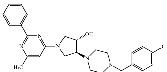
4-[4-(4-chlorobenzoyl)piperazin-1-yl]-1-(6-methyl-2-phenylpyrimidin-4-yl)pyrrolidin-3-ol
