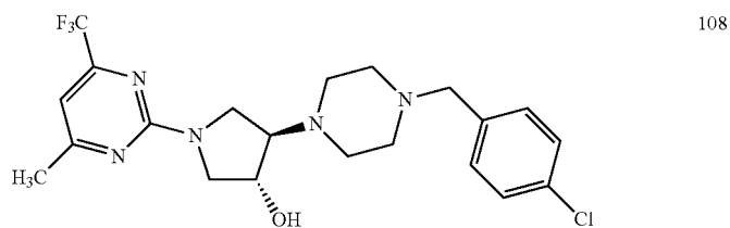
4-[4-(4-chlorobenzoyl)piperazin-1-yl]-1-[4-methyl-6-(trifluoromethyl)pyrimidin-2-yl]pyrrolidin-3-ol
