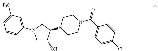
4-[4-(4-chlorobenzoyl)piperazin-1-yl]-1-[3-(trifluoromethyl)phenyl]pyrrolidin-3-ol
