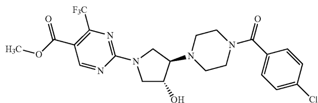
methyl 2-{3-[4-(4-chlorobenzoyl)piperazin-1-yl]-4-hydroxypyrrolidin-1-yl}-4-(trifluoromethyl)pyrimidine-5-carboxylate
