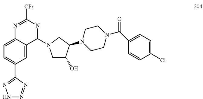
4-[4-(4-chlorobenzoyl)piperazin-1-yl]-1-[6-(2H-tetrazol-5-yl)-2-(trifluoromethyl)quinazolin-4-yl]pyrrolidin-3-ol
