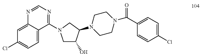
(3R,4R)-4-[4-(4-chlorobenzoyl)piperazin-1-yl]-1-(7-chloroquinazolin-4-yl)pyrrolidin-3-ol
