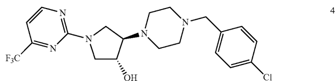
4-[4-(4-chlorobenzyl)piperazin-1-yl]-1-[4-(trifluoromethyl)pyrimidin-2-yl]pyrrolidin-3-ol
