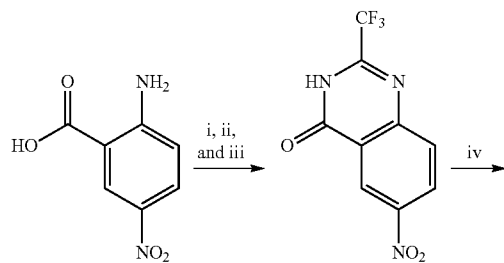
Scheme 6
