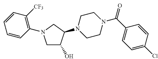
4-[4-(4-chlorobenzoyl)piperazin-1-yl]-1-[2-(trifluoromethyl)phenyl]pyrrolidin-3-ol
