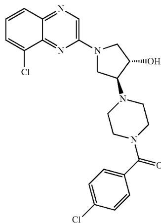
4-[4-(4-chlorobenzoyl)piperazin-1-yl]-1-(8-chloroquinoxalin-2-yl)pyrrolidin-3-ol
