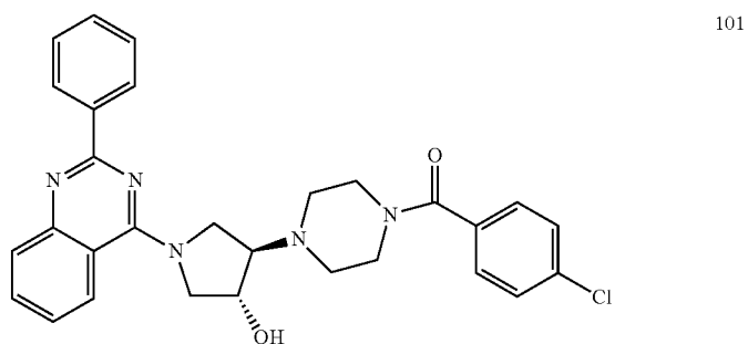
4-[4-(4-chlorobenzoyl)piperazin-1-yl]-1-(2-phenylquinazolin-4-yl)pyrrolidin-3-ol
