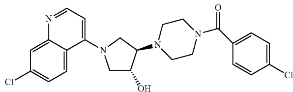
(3R,4R)-4-[4-(4-chlorobenzoyl)piperazin-1- yl]-1-(7-chloroquinolin-4-yl)pyrrolidin-3-ol
