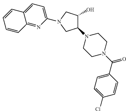
4-[4-(4-chlorobenzoyl)piperazin-1-yl]-1-quinolin-2-ylpyrrolidin-3-ol
