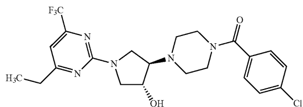
4-[4-(4-chlorobenzoyl)piperazin-1-yl]-1-[4-ethyl-6-(trifluoromethyl)pyrimidin-2-yl]pyrrolidin-3-ol
