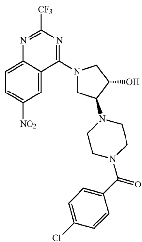
4-[4-(4-chlorobenzoyl)piperazin-1-yl]-1-[6-nitro-2-(trifluoromethyl)quinazolin-4-yl]pyrrolidin-3-ol
