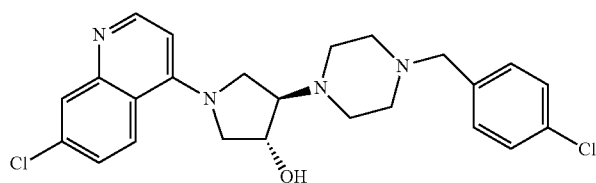
(3R,4R)-4-[4-(4-chlorobenzyl)piperazin-1- yl]-1-(7-chloroquinolin-4-yl)pyrrolidin-3-ol
