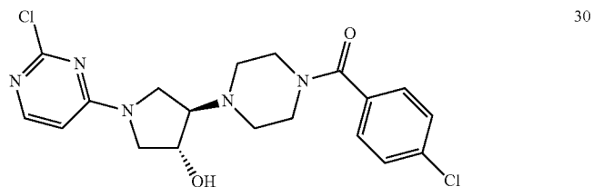
4-[4-(4-chlorobenzoyl)piperazin-1-yl]-1-(2-chloropyrimidin-4-yl)pyrrolidin-3-ol
