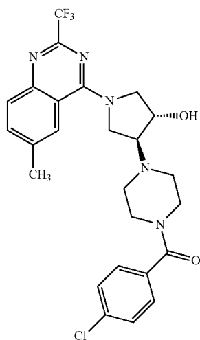
4-[4-(4-chlorobenzoyl)piperazin-1-yl]-1-[6-methyl-2-(trifluoromethyl)quinazolin-4-yl]pyrrolidin-3-ol
