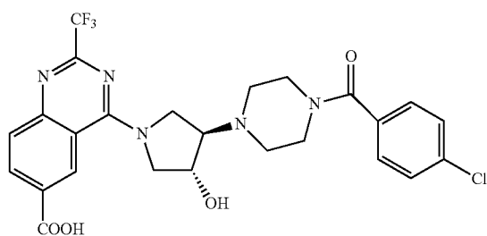
4-{3-[4-(4-chlorobenzoyl)piperazin-1-yl]-4-hydroxypyrrolidin-1-yl}-2-(trifluoromethyl)quinazoline-6-carboxylic acid
