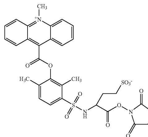
MeAE-HCA-NHS
