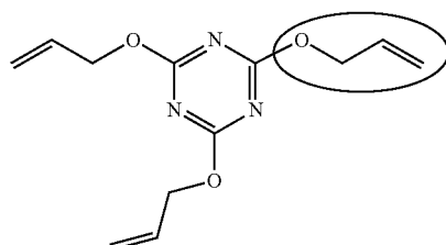
2,4,6-Triallyloxy-1,3,5-triazine
