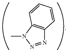
benzotriazole
