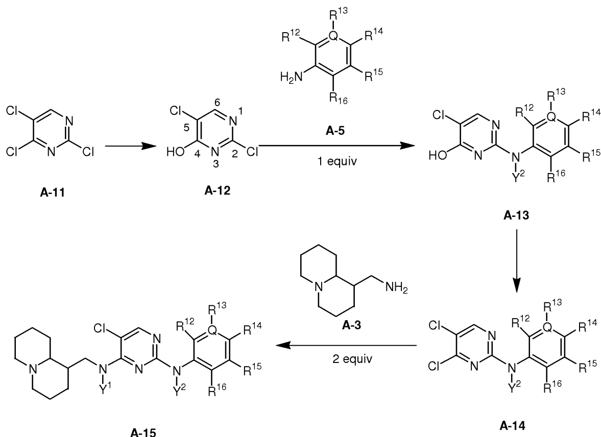
Scheme 3
