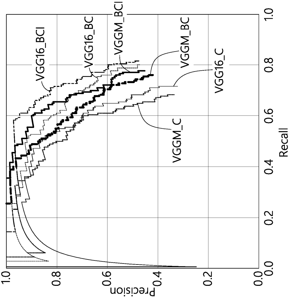
Precision-Recall Curve
