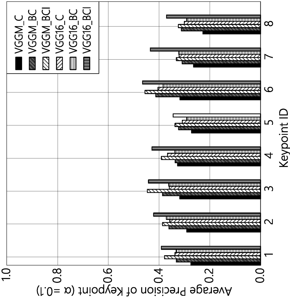
Keypoint-wise APK
