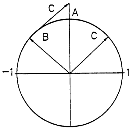
DECOMPOSITION TO TWO CONSTANT ENVELOPE SIGNALS
