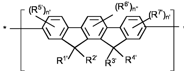
Formula (B/B')- represents cis and trans isomers
