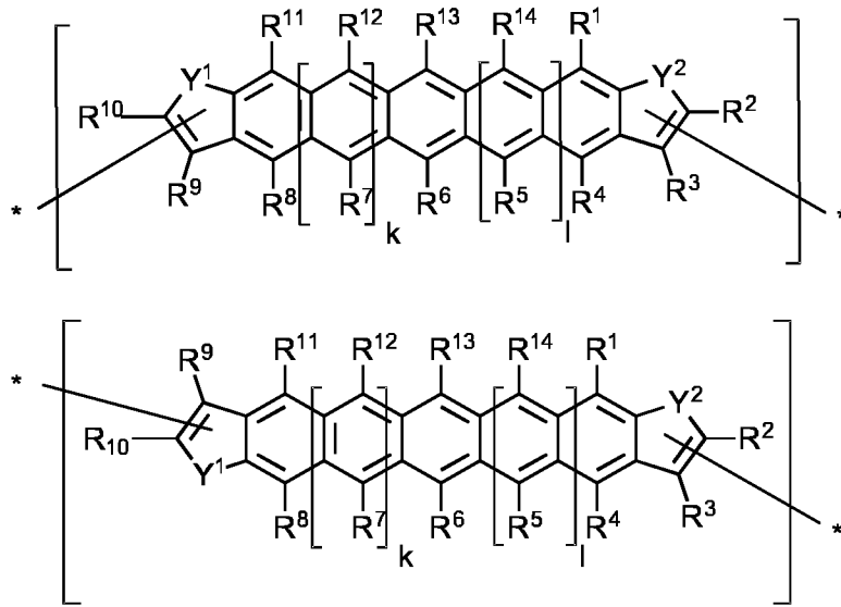
Formula (A)-represents cis and trans heteroacene
