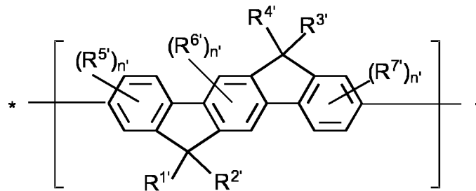
Formula (B/B')- represents cis and trans isomers
