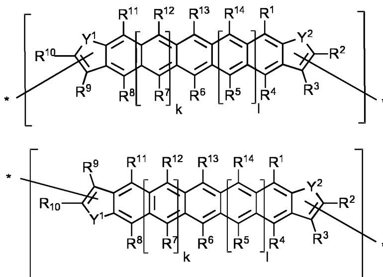
Formula (A1)-cis and/or trans isomers
