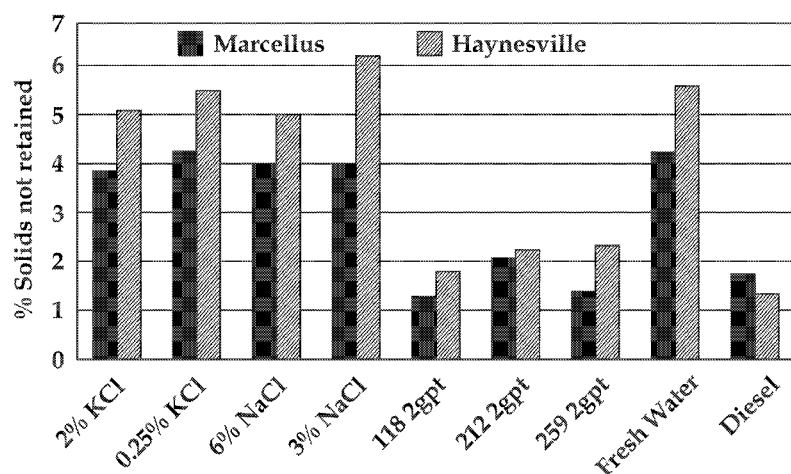
Roller Oven Shale Stability
