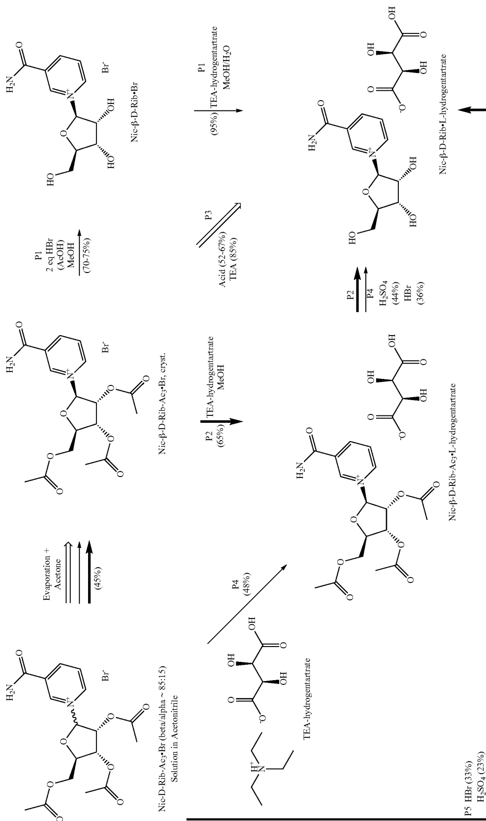
Scheme 1: Pathways to P1 to P5 for making nicotinamide- \beta -D-ribofuranoside L-hydrogen tartrate starting from nicotinamide-2,3,5-O-triacetyl- \beta -D-ribofuranoside bromide
