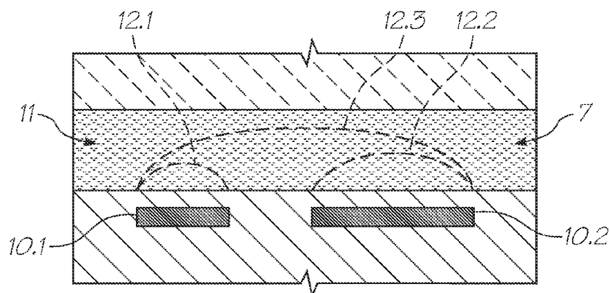
FIG. 52 (PRIOR ART)
