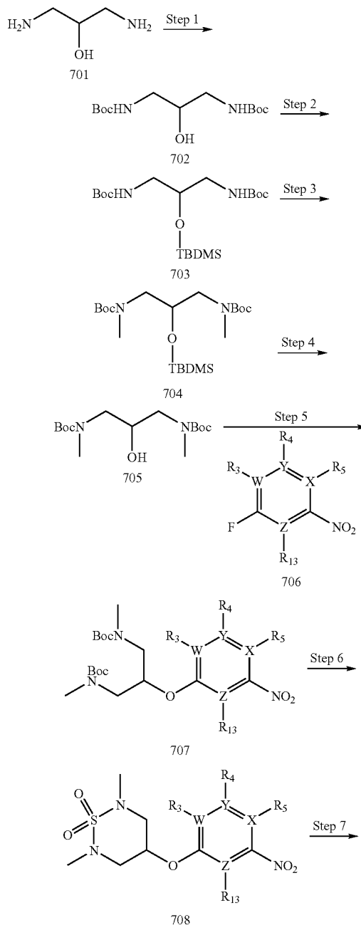
Reaction Scheme 7
