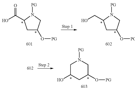
REACTION SCHEME 6
