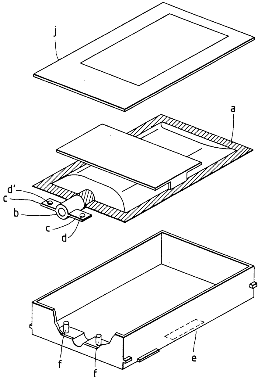
FIG. 7 PRIOR ART
