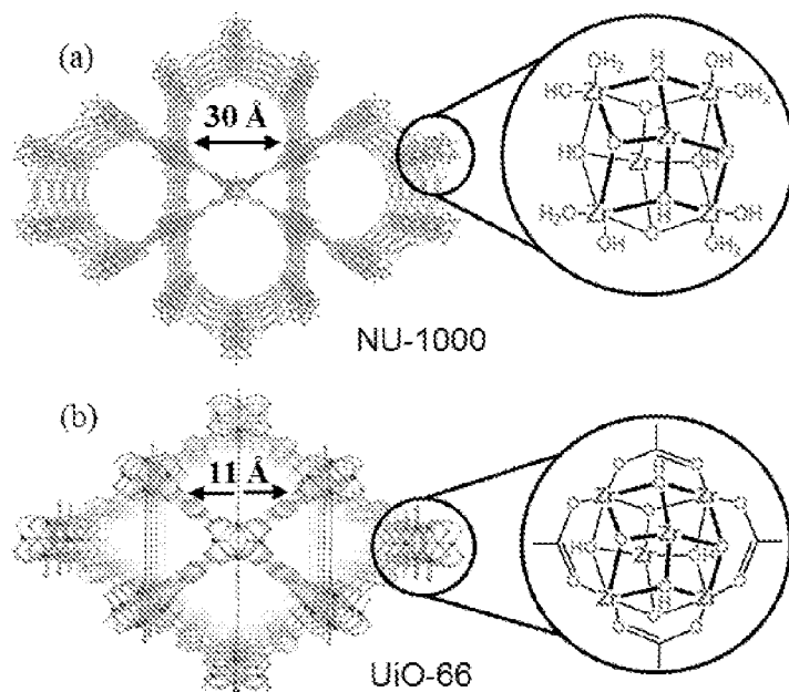
Figure 4. (a) Structure of NU-1000 highlighting the hexagonal pore size and the structure of the Zr 6 node. (b) Structure of UiO-66 highlighting the octahedral pore size and the structure of the Zr 6 node.
