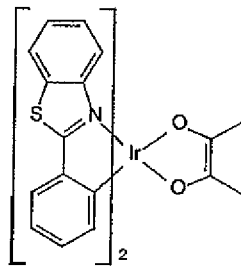
Bt 2 (acac)
